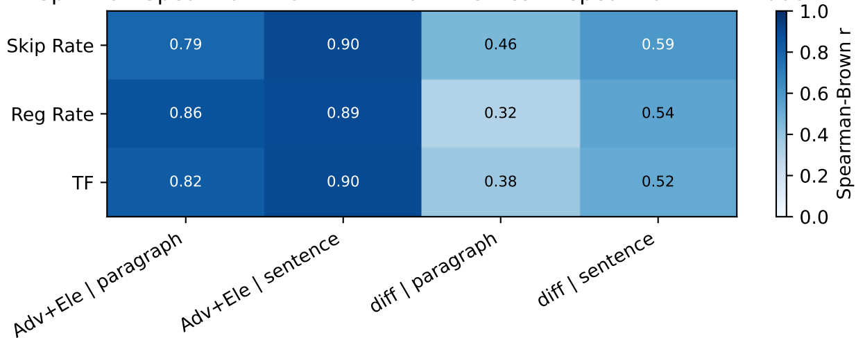
Split-half Spearman-Brown r — main metrics — spearman — N=1000
