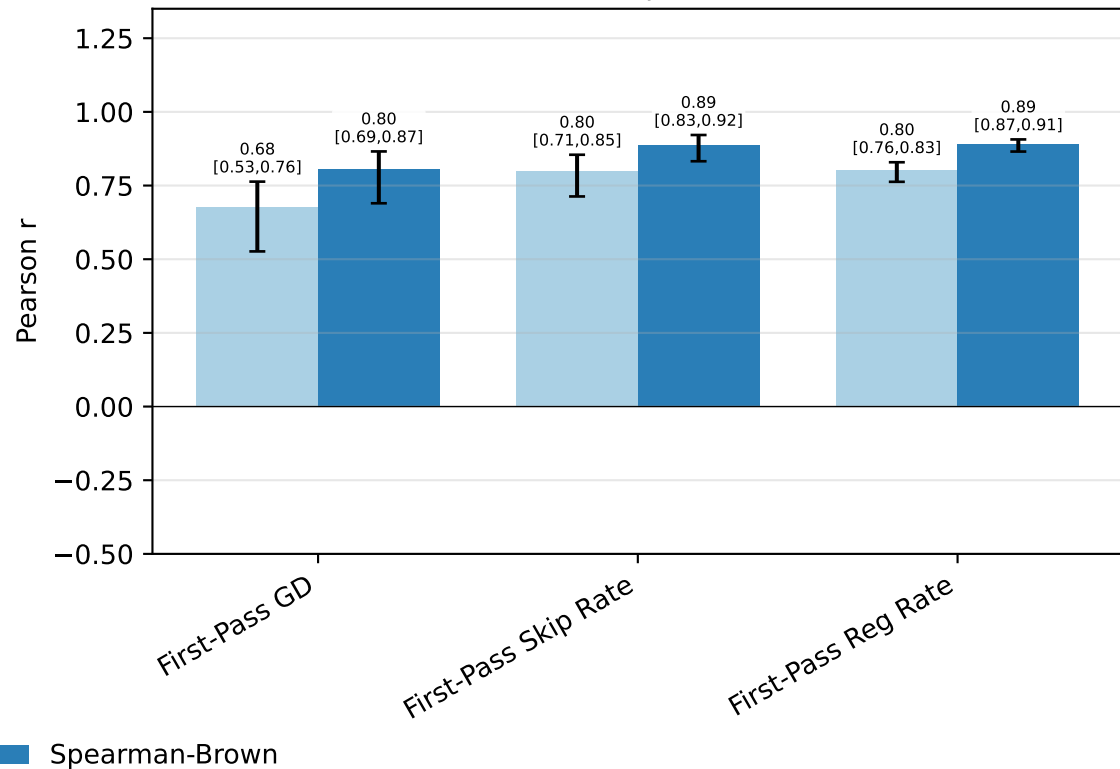
Sentence | Pearson
