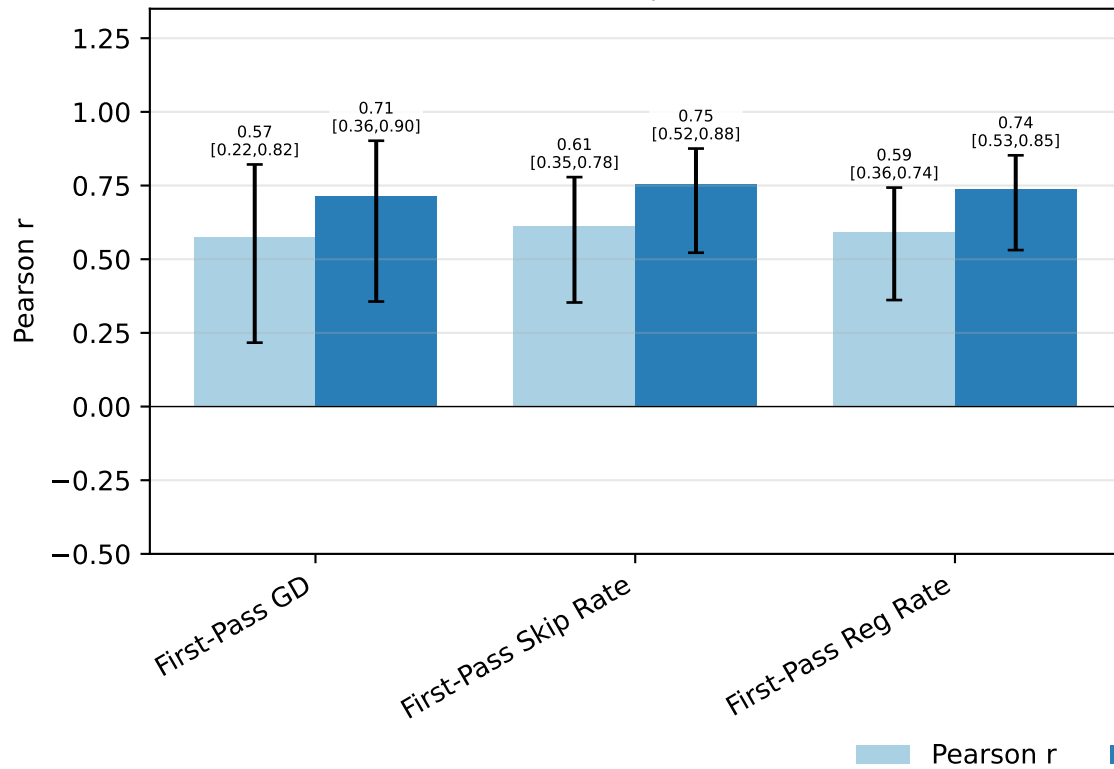
Paragraph | Pearson
