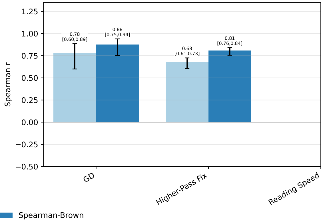
Sentence | Spearman
