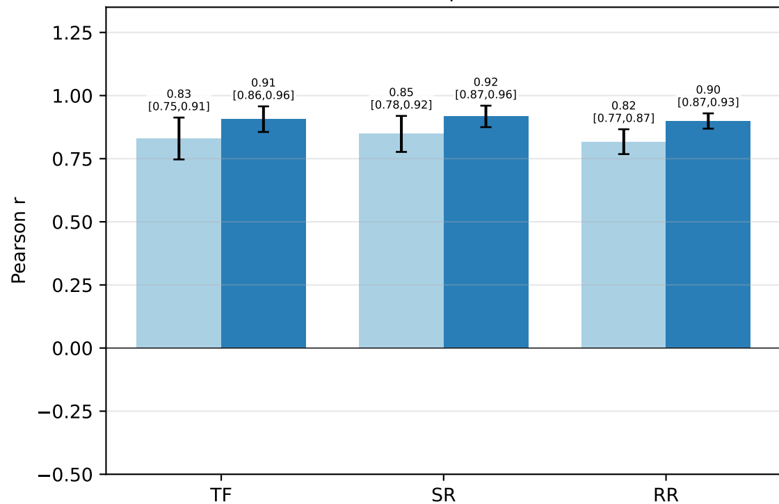
Sentence | Pearson
