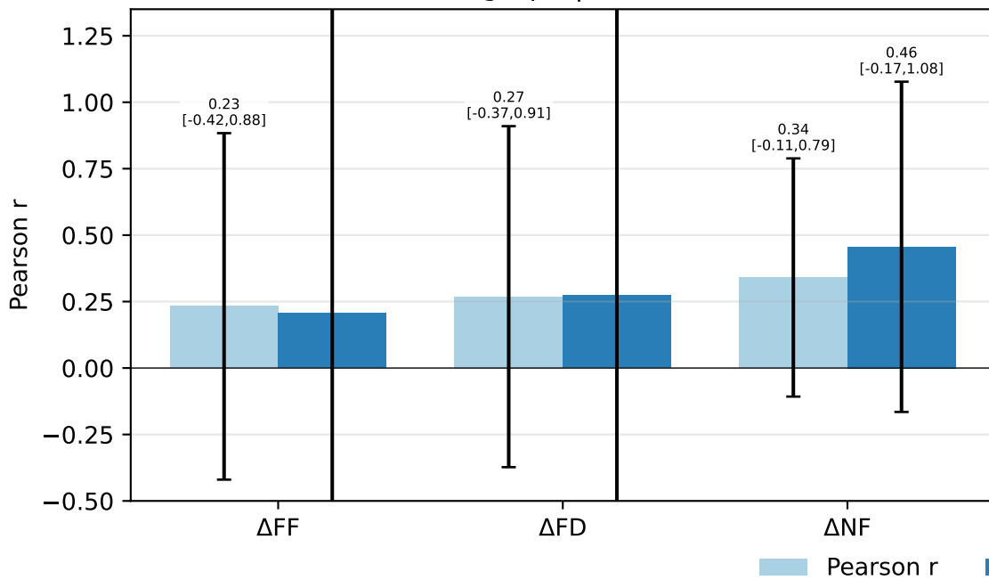
Paragraph | Pearson
