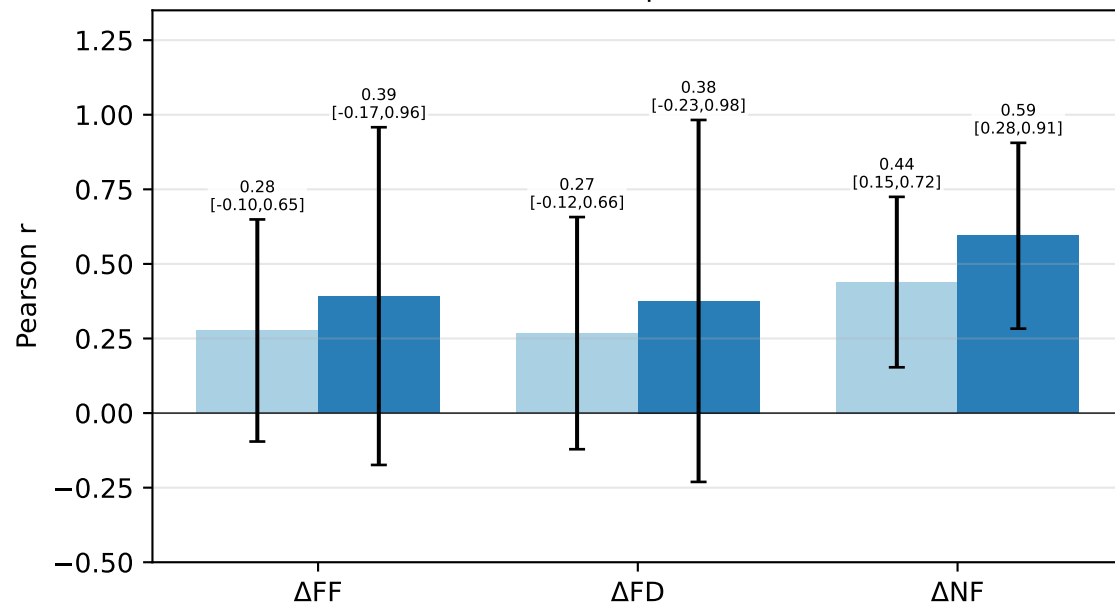
Sentence | Pearson
