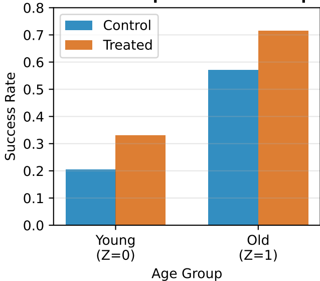
Within Groups: Treatment Helps
