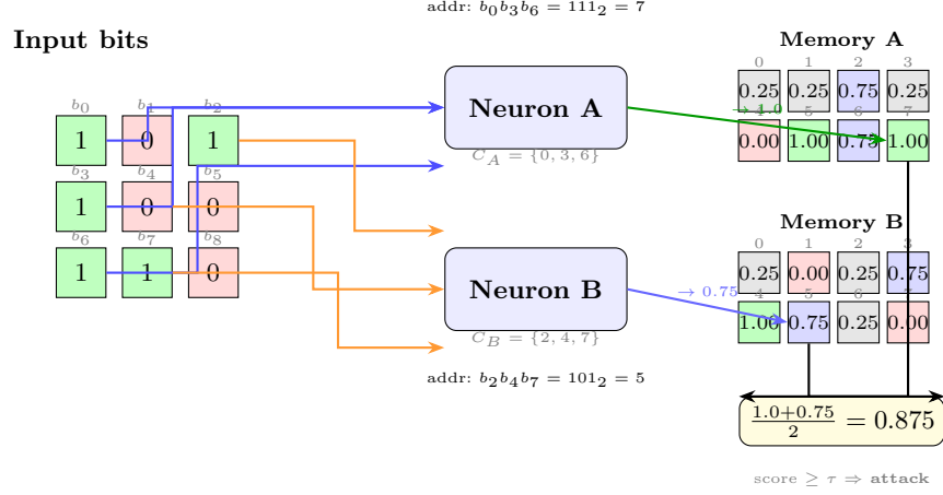
Fig. 1. RAM neuron architecture with two neurons ( N=2 , n=3 address bits each). Each neuron selects 3 bits from the 9-bit input via its connectivity map, forms a 3-bit address, and looks up its quad-weighted memory ( 2^3=8 cells). Cell colors: TRUE (1.0), WEAK_TRUE (0.75), WEAK_FALSE (0.25), FALSE (0.0). The mean score is thresholded to classify the input.
