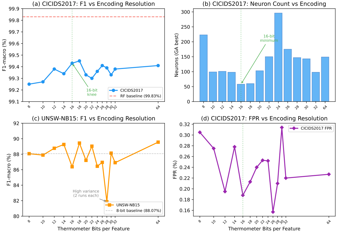
Figure 2. Effect of thermometer encoding resolution on classification performance. (a) CICIDS2017 F1 shows a clear knee at 16 bits, with diminishing returns beyond. (b) The GA finds the fewest neurons at 16 bits, suggesting optimal information density. (c) UNSW-NB15 temporal split shows no clear trend (high variance from only 2 runs per configuration). (d) CICIDS2017 false positive rate is lowest around 16–26 bits.
