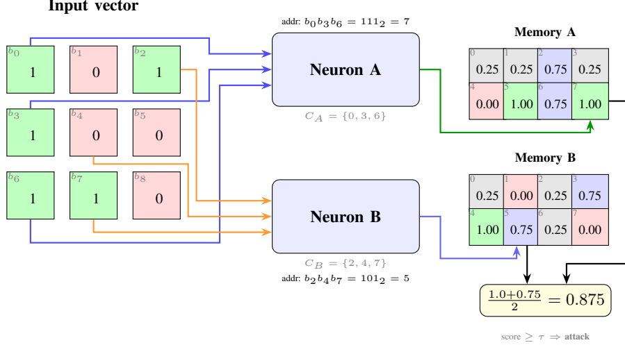
Figure 1. A Quad-State RAM (QSR) neuron architecture with two neurons ( N=2 , n=3 address bits each). Each neuron selects 3 bits from the 9-bit input via its connectivity map, forms a 3-bit address, and looks up its QSR memory ( 2^3=8 cells). Cell colors: TRUE (1.0), WEAK_TRUE (0.75), WEAK_FALSE (0.25), FALSE (0.0). The mean score is thresholded to classify the input.
