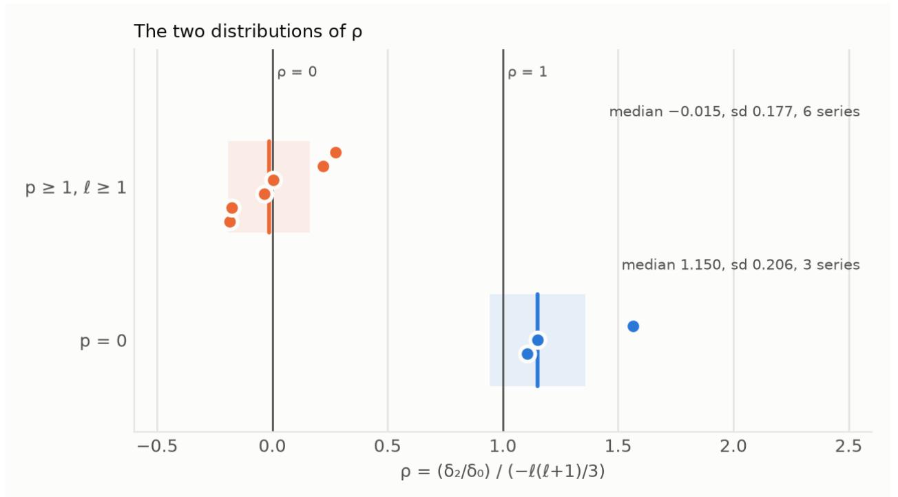
Figure 1. (a) The fitted ratio \delta_2/\delta_0 of all thirteen series against p , with the polarisation value -\ell(\ell+1)/3 drawn for \ell = 0, 1, 2, 3 . (b) \rho against p for the nine series with \ell \geq 1 : the p = 0 class at median 1.150 with the \pm 0.206 band, the p \geq 1 class at median -0.015 with the \pm 0.177 band.
