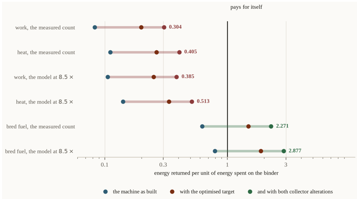
Figure 4. The range the reaction is expected to fall in. Each row is one way of pricing the same reaction; the bar runs from what the machine as built delivers to what it delivers with all three alterations. Anything reaching the line at unity pays for itself. Only bred fuel does, and the rows at the measured cycle count use no service-life model at all.
