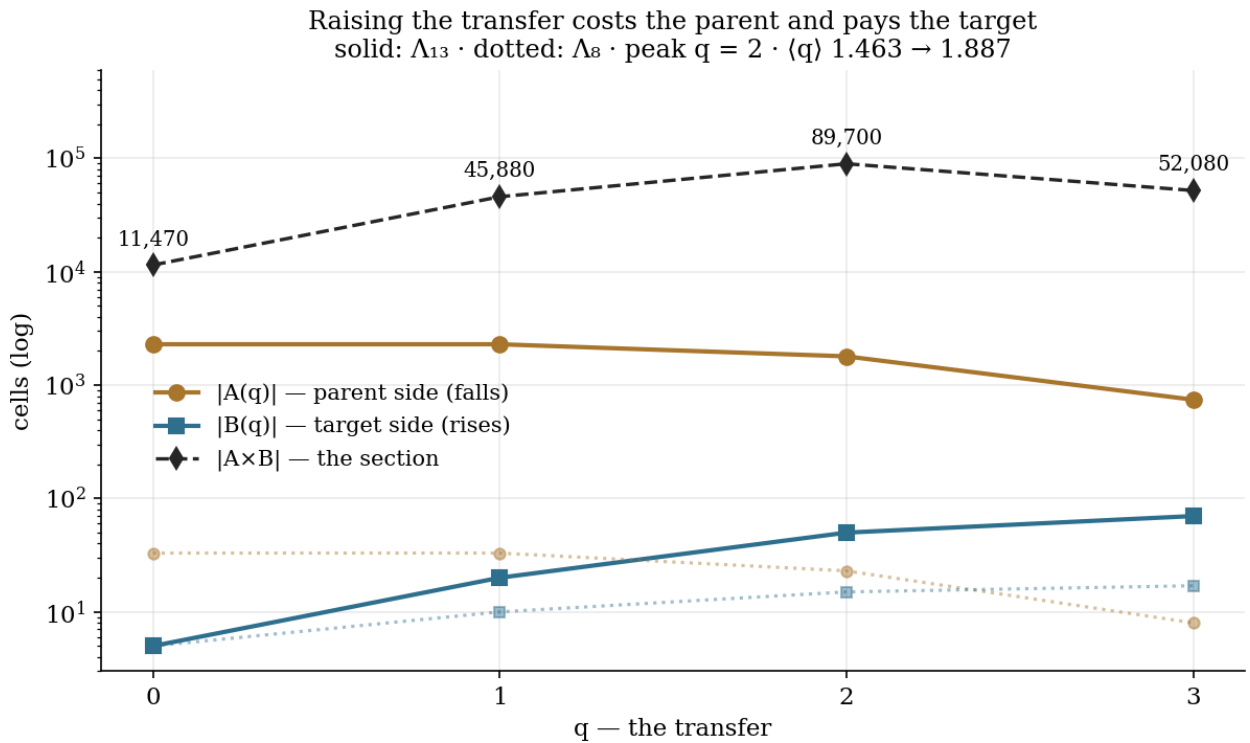
Figure 12.3. The Pareto frontier on a log axis, \Lambda_{13} solid against \Lambda_8 dotted: A falls and B rises at both scales, and no q improves both. The section |A \times B| peaks at q = 2 with 89,700 cells, and the tower shifts \langle q \rangle from 1.463 to 1.887 — coupling multiplicity re-weights the profile toward higher transfer, per §12.11.5.
