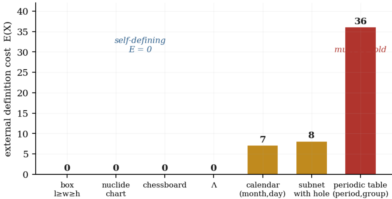
Figure 6.1. The external definition cost of seven indices. Four are self-defining. The calendar's seven cells are the content of Thirty days hath September; the periodic table's thirty-six are the gaps in the short periods.
