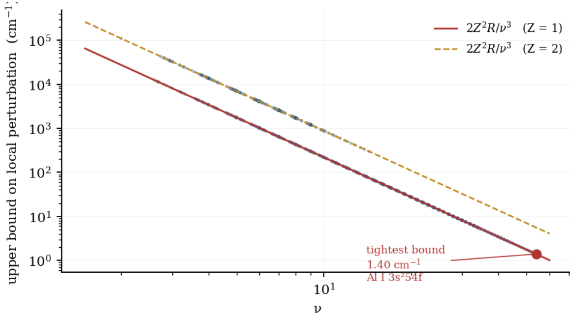
Figure 25.1. Each of the 1,061 cells that yield a perturbation bound, plotted at the bound its containment implies. The two curves are the failure condition at Z = 1 and Z = 2 . Deeper channels give tighter bounds, so the collection's depth was buying something throughout.
