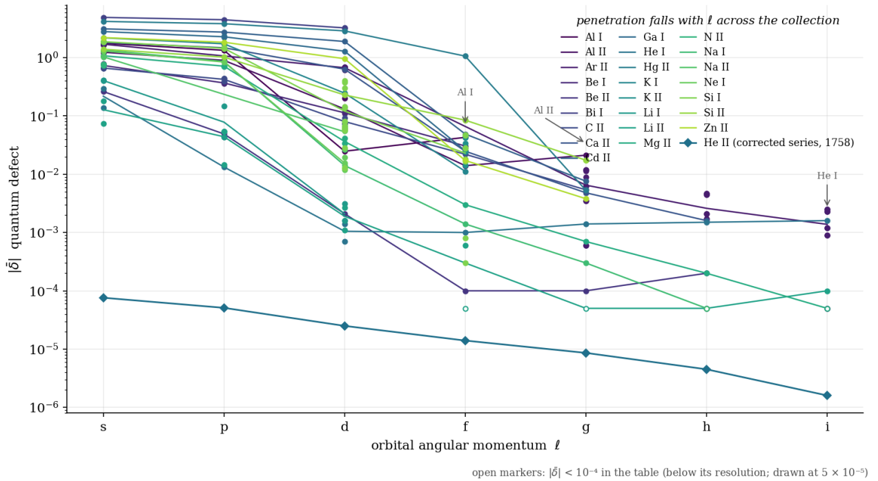
Figure 24.1. Every species in the collection, defect against angular momentum. The fall is monotone in every species wherever the defect is the core's, and spans six orders of magnitude — from 4.9 in bismuth to 1.6 \times 10^{-6} in He II. The three places it rises are marked, and none is penetration: Al I nd and Al II nf are two of the channels §B.3 flags as perturbed, and He I above d sits on its fine-structure floor near 10^{-3} , where what remains is not the core.
