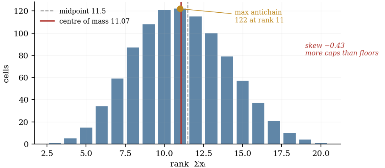
Figure 8.2. The rank sequence over all 976 cells is log-concave, hence unimodal, hence Sperner. It is not symmetric: the centre of mass sits below the midpoint by 0.43, because \Lambda has more caps than floors.
