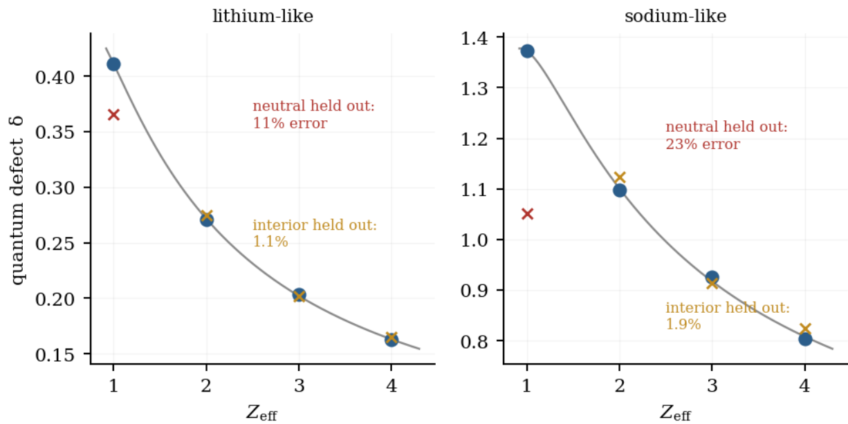
Figure 24.3. Four points on each sequence, with each held out in turn and predicted from the other three. Crosses are predictions; circles are measurements. The interior is recovered to about one percent. The neutral is not.
