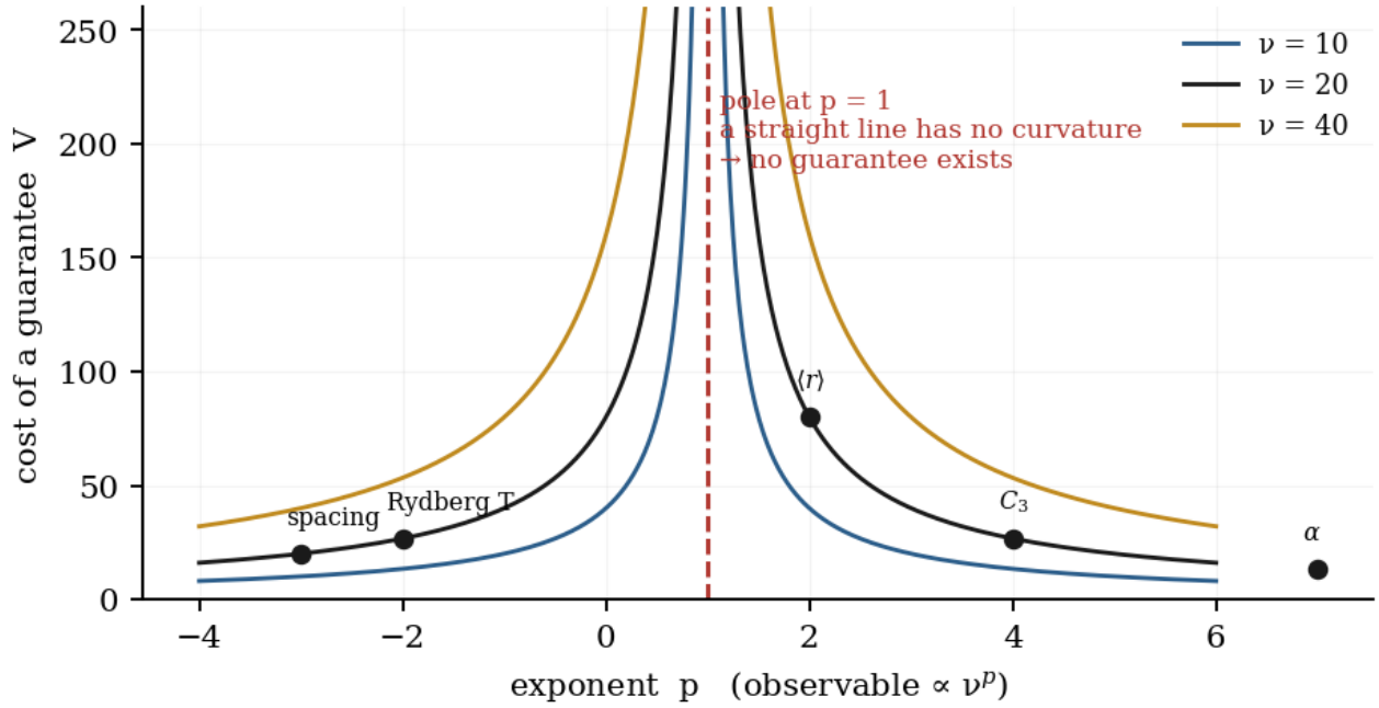
Figure 23.2. The cost surface. Every observable in this book is a slice at fixed p . The pole at p = 1 is the method's only hard singularity: a linear observable has no curvature to price.
