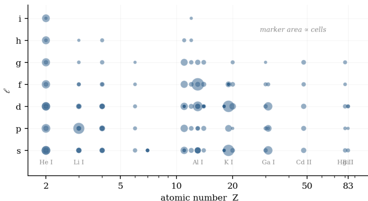
Figure 24.2. What the collection covers. Marker area is proportional to cells. The gaps are not omissions: the census of §24.12 excludes them structurally.
