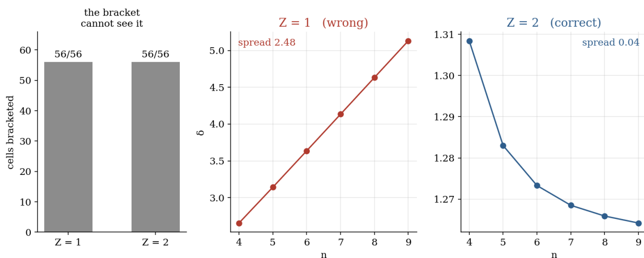
Figure 16.1. The bracket holds fifty-six of fifty-six under either charge, because Z cancels from containment. The defect does not: at Z = 1 it spreads over several units, which no Rydberg series can do. The method was blind; a quantity the method never uses was not.
