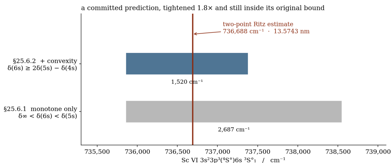
Figure 25.2. The Sc VI prediction as it now stands. §25.6.1's bracket uses monotonicity alone — \delta decreasing gives \delta_\infty < \delta(6s) < \delta(5s) , a width of 2,687 \text{cm}^{-1} . §25.6.2 adds convexity: \delta = \delta_0 + \delta_2/n^2 lies above its own tangent, so \delta(6s) \geq 2\delta(5s) - \delta(4s) = 0.9567 , narrowing the interval to 1,520 \text{cm}^{-1} without leaving it. The two-point Ritz estimate sits inside both. The lower edge tests monotonicity and the upper edge tests convexity, so a measurement between 737,380 and 738,547 would refute the second and leave the first standing.
