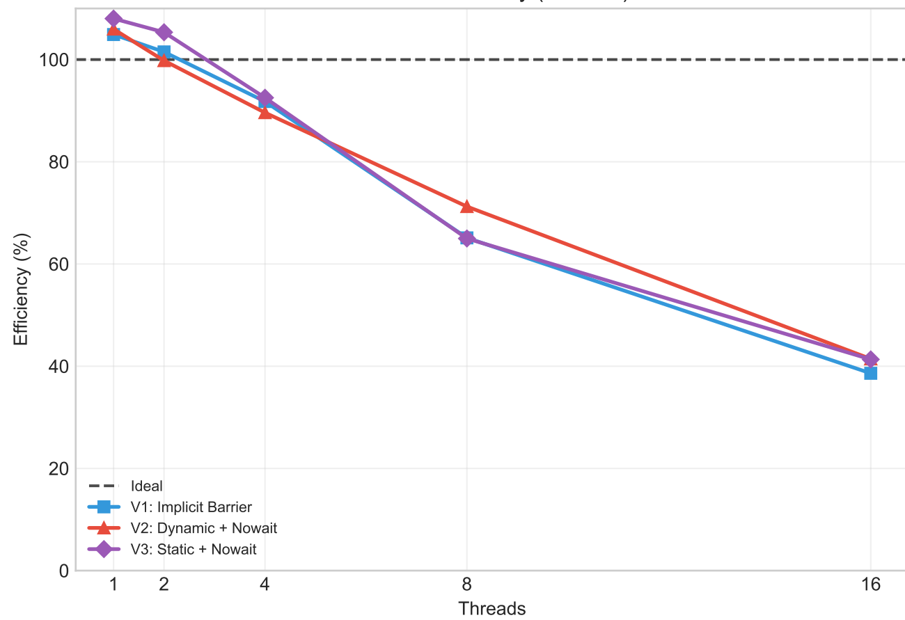
Parallel Efficiency (N=2000)
