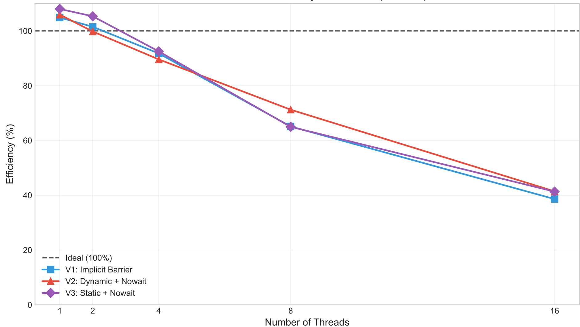
DMVM Parallel Efficiency vs Threads (N=2000)
