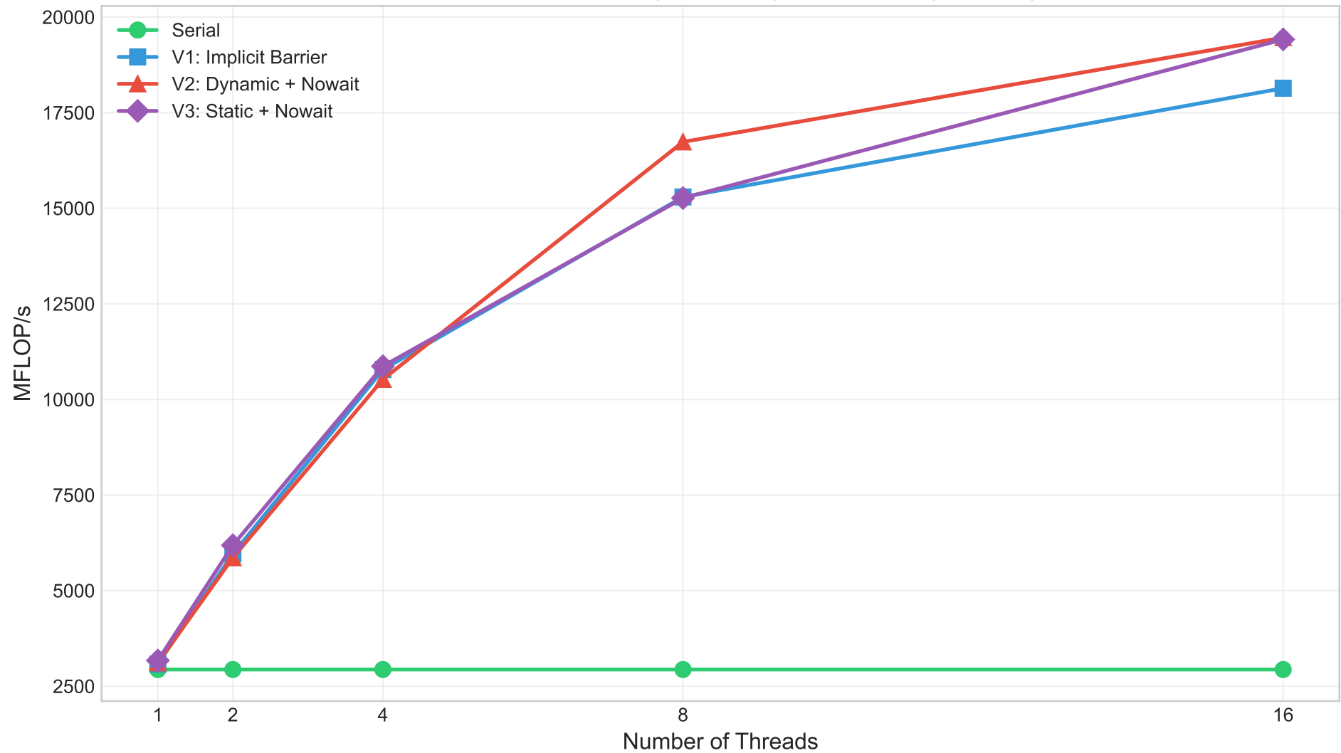
DMVM Performance (MFLOP/s) vs Threads (N=2000)
