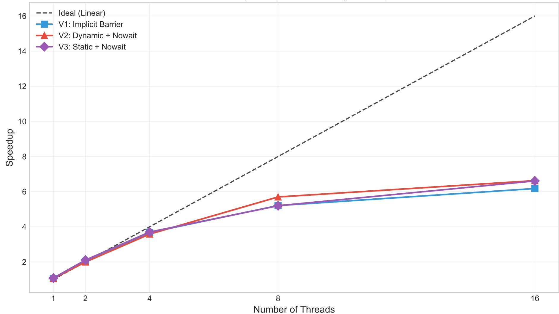
DMVM Speedup vs Threads (N=2000)
