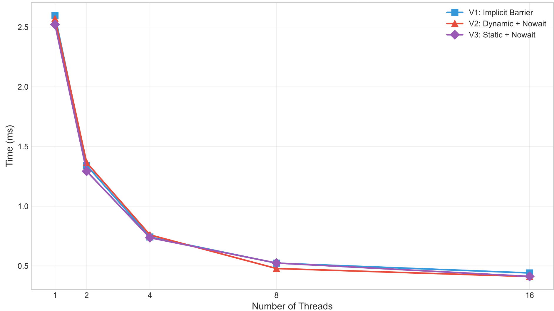
DMVM Execution Time vs Threads (N=2000)
