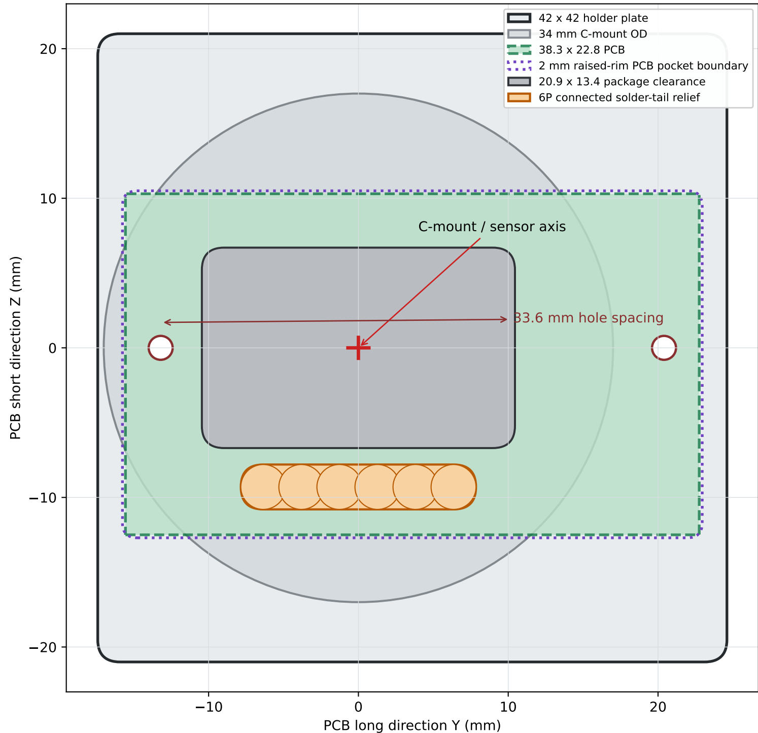
C12880MA module holder: rear alignment (looking toward C-mount)
