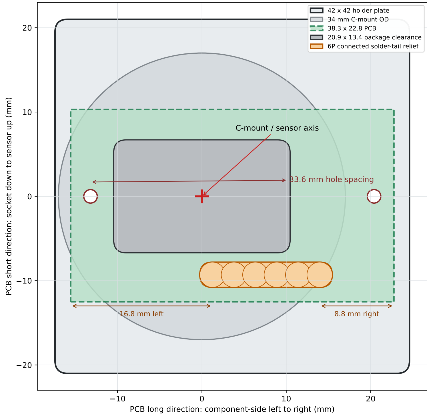
C12880MA component-side top view: sensor up, socket down
