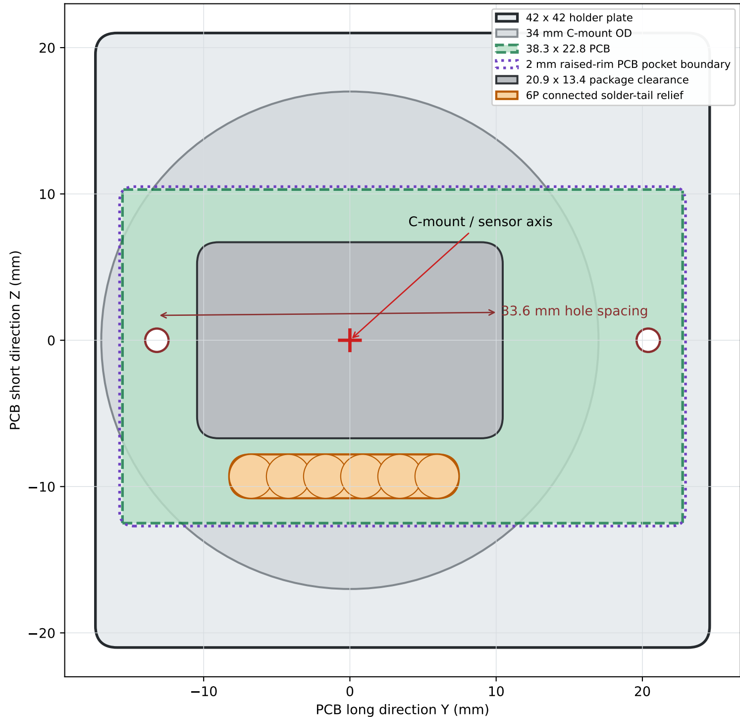
C12880MA holder: component-side alignment (sensor up, socket down)
