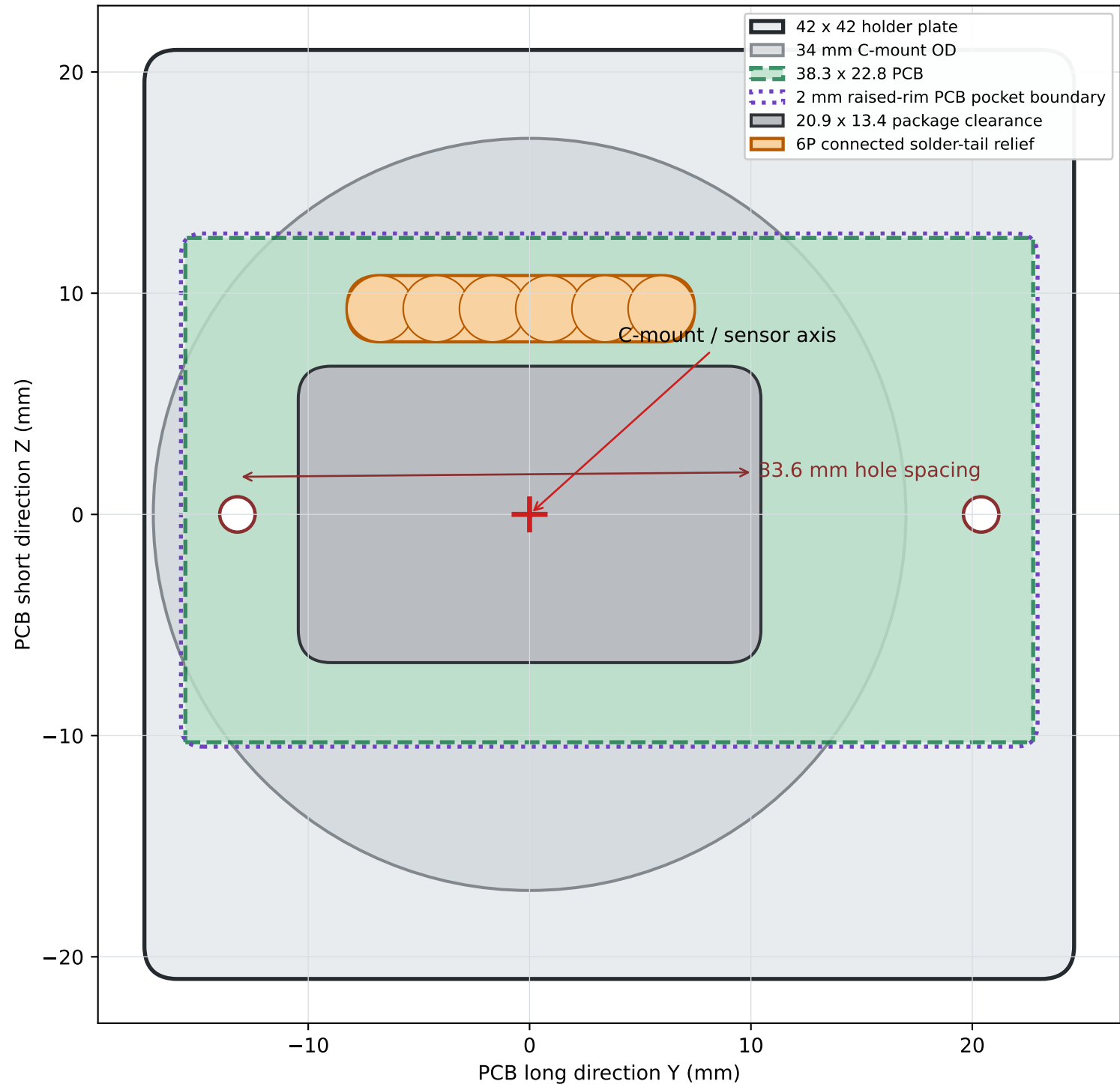
C12880MA holder mating face: source short direction inverted
