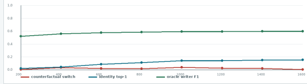
Figure 10: Measured V22 result. Actual endpoint samples show that targets switch when only the final visual query changes, while candidate predictions barely move and match the query-blind control. The candidate selector assigns every one of 1,024 development argmaxes to the operation frame. Writer metrics improve without relational prompt binding.
