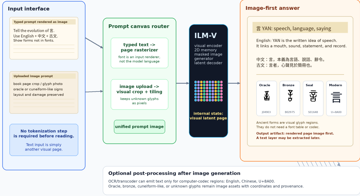
Figure 13: Inference pipeline for ILM-V. A chat-like interface may accept typed text or uploaded images, but typed text is first rasterized into a prompt image. The primary output is a rendered page image. OCR or transcoding is optional and only applies to output regions that exist in computer codecs.
