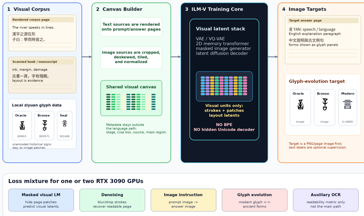
Figure 12: Training pipeline for ILM-V. Rendered text corpora, scanned pages, historical glyph files, and unencoded marks are all converted into visual canvases. The training target is visual latent prediction and image generation, not BPE-token prediction.
