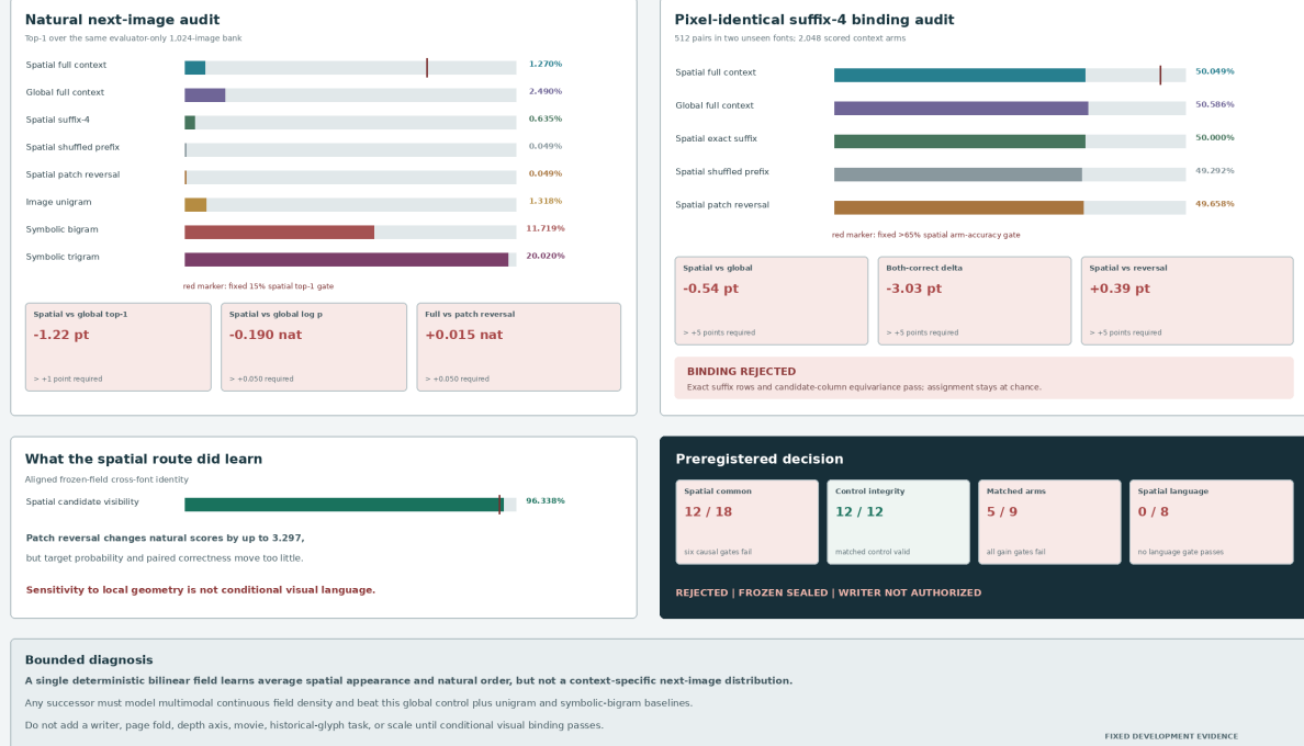
Figure 19: Measured V30 matched-arm result generated directly from the fixed audit. The spatial route is sensitive to local candidate alignment but is worse than the parameter-identical global route on natural top-1, target log probability, pair assignment, and pair both-correct. It passes 12/18 common gates and 0/8 language gates; the control passes all 12 integrity gates.
