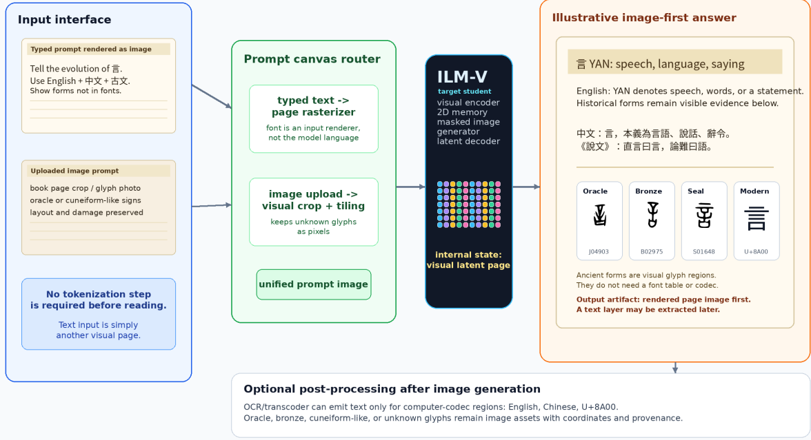
Figure 30: Proposed inference contract for ILM-V. A chat-like interface may accept typed text or uploaded images, but typed text is first rasterized into a prompt image. The target primary output is a rendered page image. OCR or transcoding is optional and applies only to output regions represented by computer codecs. The displayed answer is illustrative, not a V30 output.
