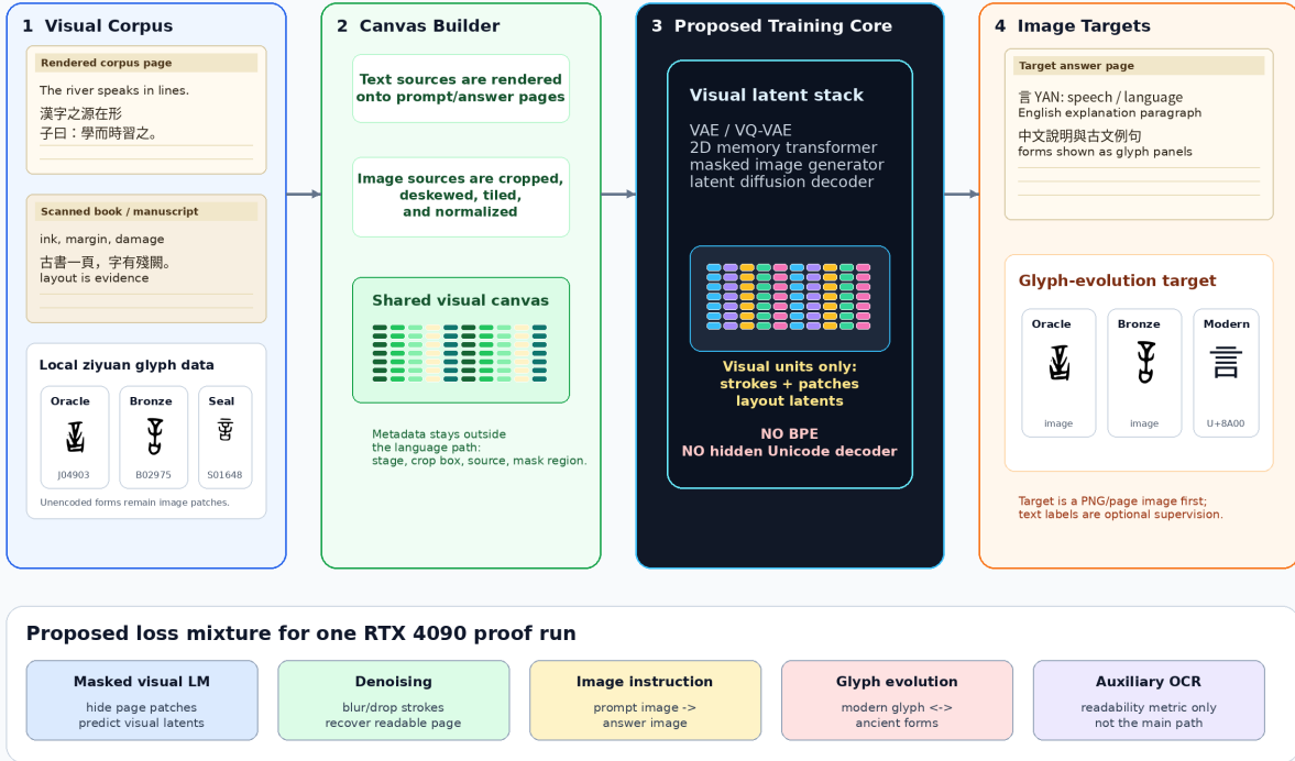
Figure 28: Proposed full-system training target for ILM-V. Rendered text corpora, scanned pages, historical glyph files, and unencoded marks become visual canvases. The intended objective predicts visual latents and images, not BPE tokens. This is a design figure; Figure 19 reports the measured reader experiment.
