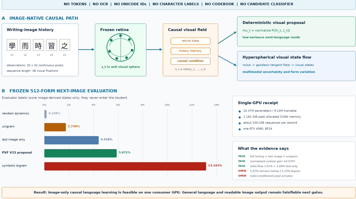
Figure 4: Measured PVF V15 state proof. Both deterministic proposal and stochastic hyperspherical field use full image history and beat random, last-only, and unigram controls. The proposal remains below the symbolic bigram, and no pixel actuator is present.
