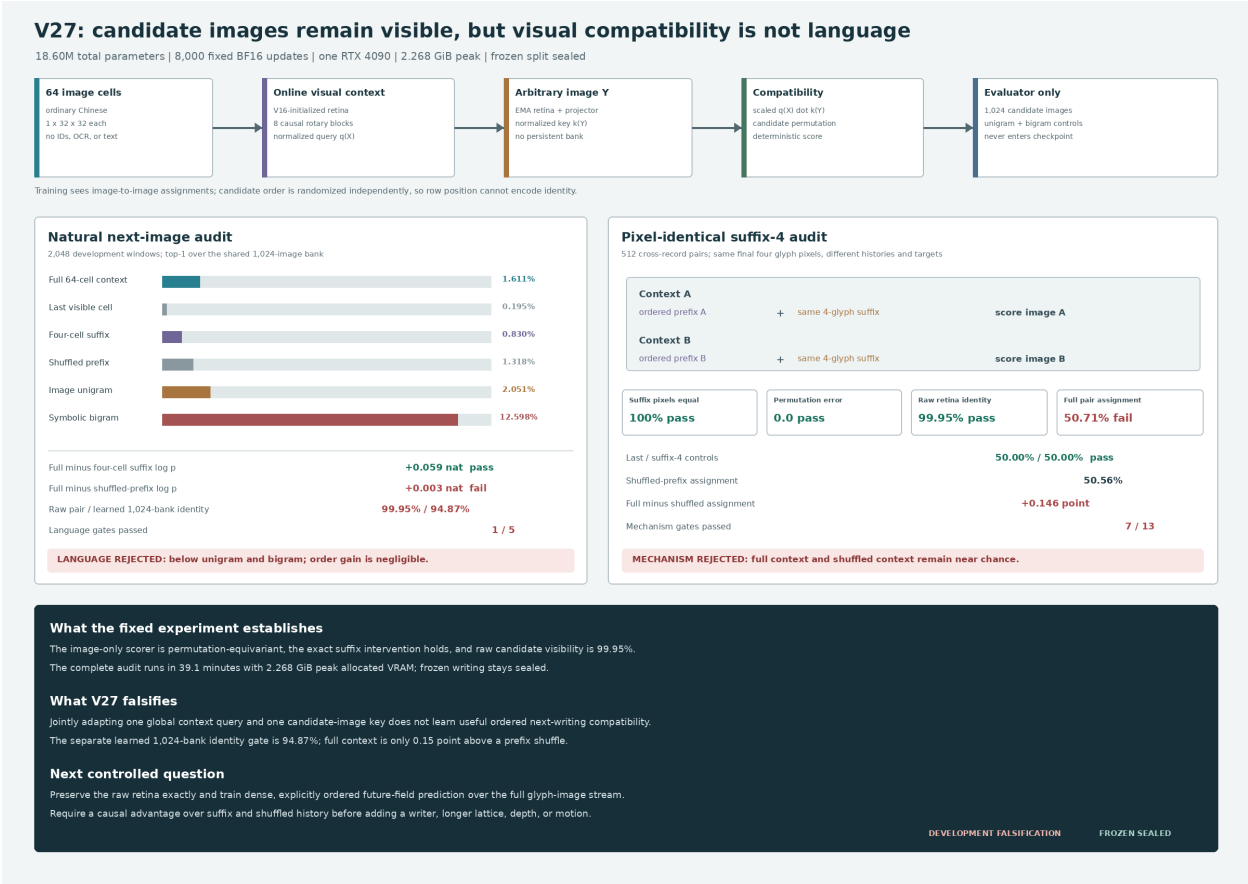
Figure 16: Measured V27 development result generated directly from the fixed audit. The image-only boundary, candidate permutation, exact suffix intervention, and raw-retina identity controls pass. Jointly learned visual compatibility remains near chance, misses its separate full-bank identity gate, and does not use prefix order. The frozen partition stays sealed and no writer is trained.
