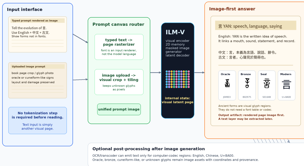
Figure 18: Inference pipeline for ILM-V. A chat-like interface may accept typed text or uploaded images, but typed text is first rasterized into a prompt image. The primary output is a rendered page image. OCR or transcoding is optional and only applies to output regions that exist in computer codecs.
