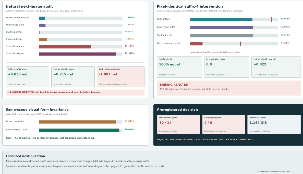
Figure 17: Measured V28 development result generated directly from the fixed audit. Frozen raw geometry and the learned semantic route preserve candidate visibility, and ordered history affects probability and mean margin. Natural selection remains below frequency controls and matched pair assignment stays at chance. Ten of fourteen mechanism gates and two of six language gates pass, so frozen evaluation and writer training remain unauthorized.
