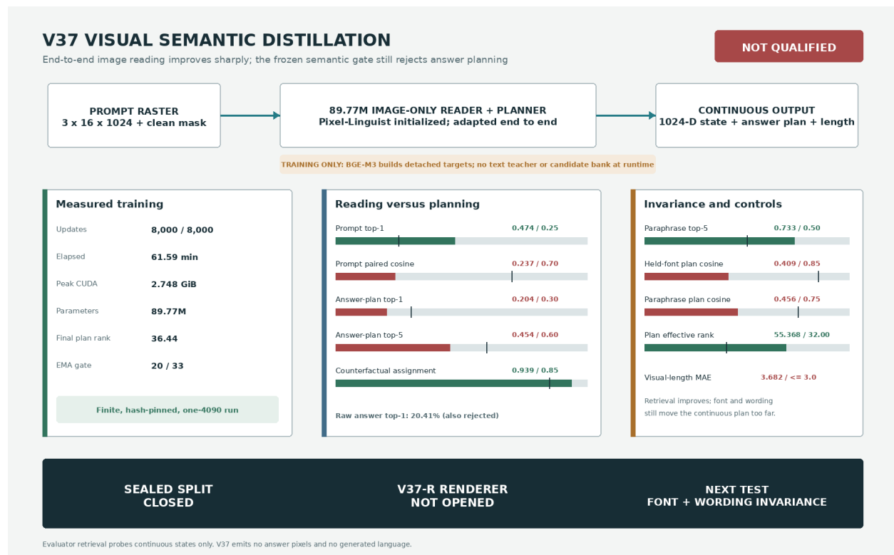
Figure 26: Measured V37 development decision generated from tracked, hash-pinned training and EMA/raw evaluation receipts. Pixel-Linguist is external initialization and BGE-M3 is an offline target builder; neither is claimed as project work or called by the deployed student. V37 predicts continuous states and does not emit answer pixels.
