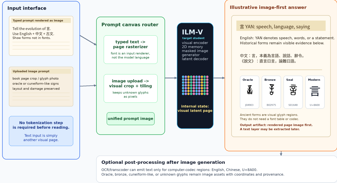
Figure 34: Proposed inference contract for ILM-V. A chat-like interface may accept typed text or uploaded images, but typed text is first rasterized into a prompt image. The target primary output is a rendered page image. OCR or transcoding is optional and applies only to output regions represented by computer codecs. The displayed answer is illustrative, not a V30 output.
