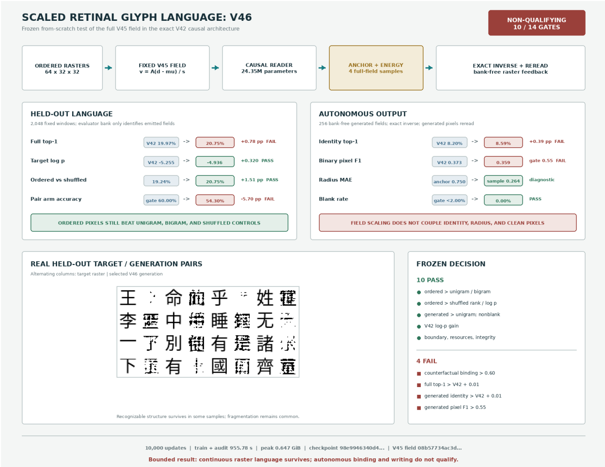
Figure 32: Measured V46 result generated deterministically from hash-pinned training and development receipts and the real target/generated raster sheet. V46 preserves ordered-raster controls and improves V42 target log probability, but its top-1 and generated-identity gains are too small, counterfactual binding remains below 0.60, and generated pixel F1 declines. The four failures make the 10/14 decision non-qualifying.
