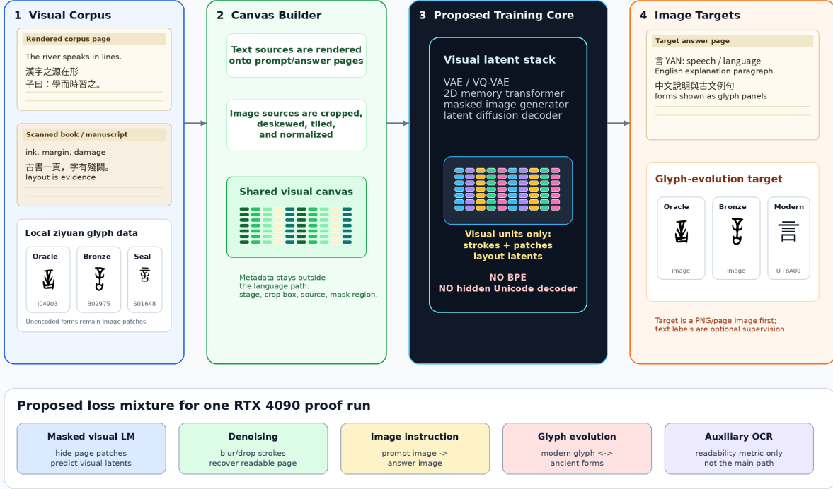
Figure 22: Proposed full-system training target for ILM-V. Rendered text corpora, scanned pages, historical glyph files, and unencoded marks become visual canvases. The intended objective predicts visual latents and images, not BPE tokens. This is a design figure; Figure 19 reports the measured reader experiment.
