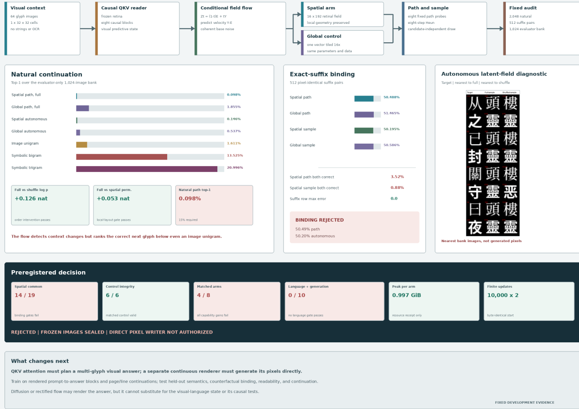
Figure 20: Measured V31 matched-arm result generated directly from the fixed audit. Conditional flow detects order, local layout, diversity, and context dependence while failing next-glyph identity and exact-suffix assignment. The embedded glyph columns are evaluator-nearest images to generated latent fields, not direct generated pixels.
