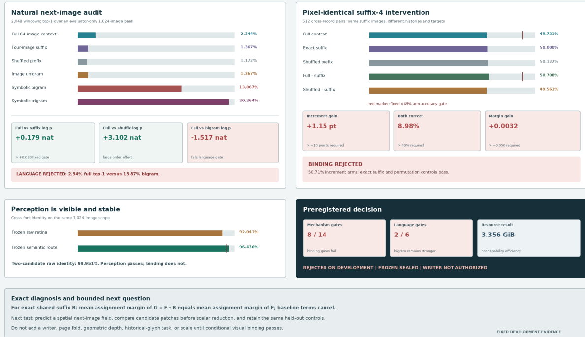
Figure 18: Measured V29 development result generated directly from the fixed audit. The critic detects a large natural order effect while exact-suffix candidate binding stays at chance. All perception, equality, permutation, leakage, and resource controls pass. Eight of fourteen mechanism gates and two of six language gates pass, so frozen evaluation and writer training remain unauthorized.
