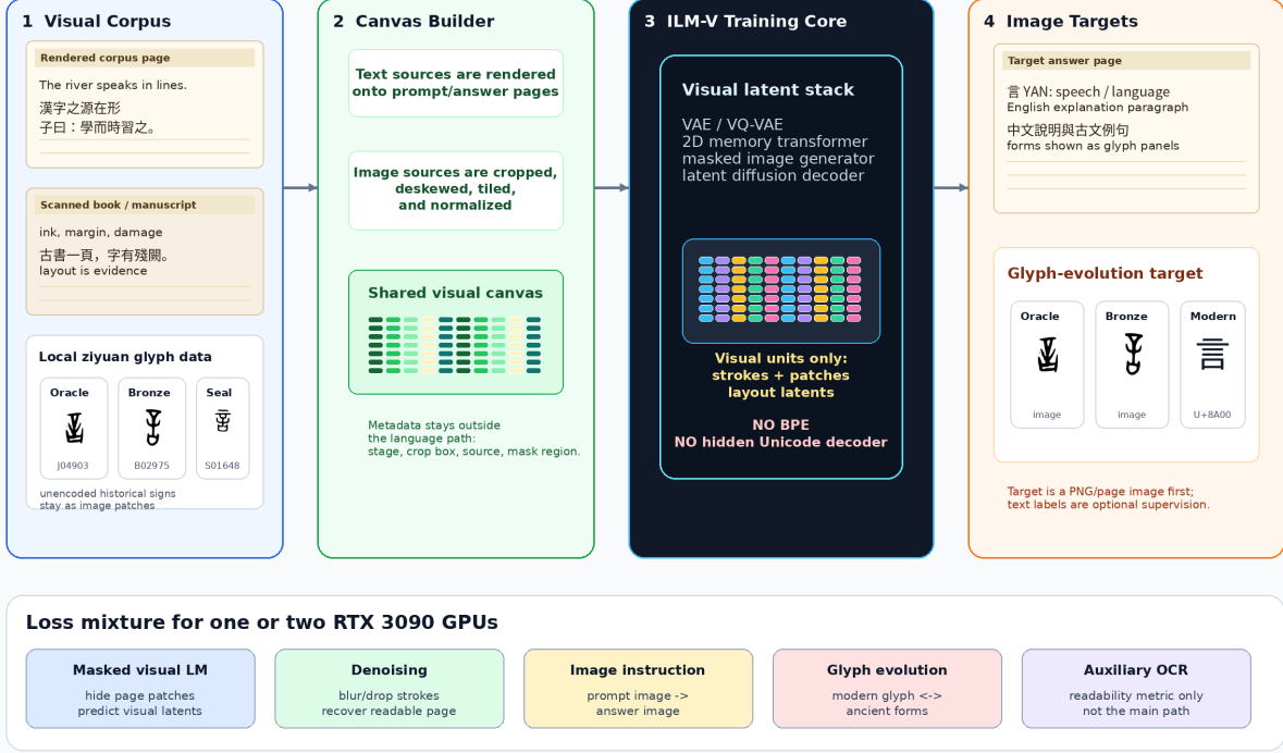
Figure 19: Training pipeline for ILM-V. Rendered text corpora, scanned pages, historical glyph files, and unencoded marks are all converted into visual canvases. The training target is visual latent prediction and image generation, not BPE-token prediction.
