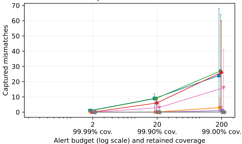
Secondary: PyMatching mismatch Captured mismatches
