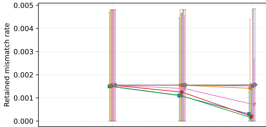
Primary: correlated-matching mismatch Retained mismatch rate
