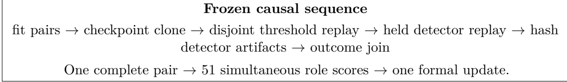
Figure 1: Protocol timeline. Threshold-state updates do not flow into held monitoring, and outcome labels cannot affect detector scores or ties.
