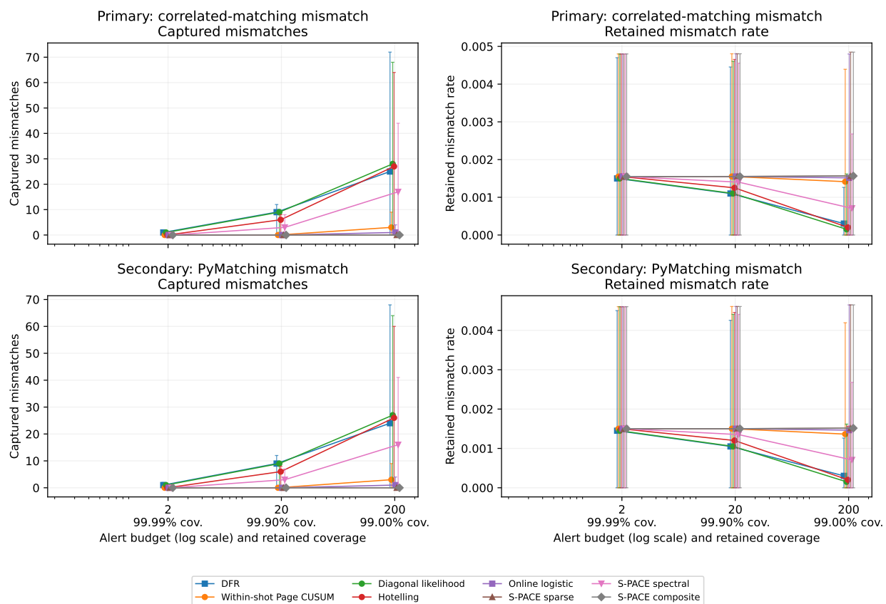
Figure 3: Retrospective utility of detector-only frozen rankings.
