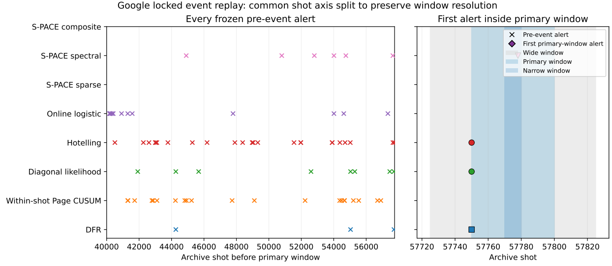
Figure 2: Google natural-event causal replay. The author-provided event location is approximate; the plot does not define an exact onset.
