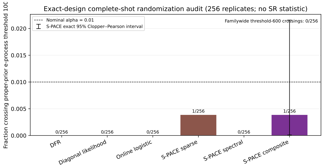
Figure 4: Exact-design randomization audit.
