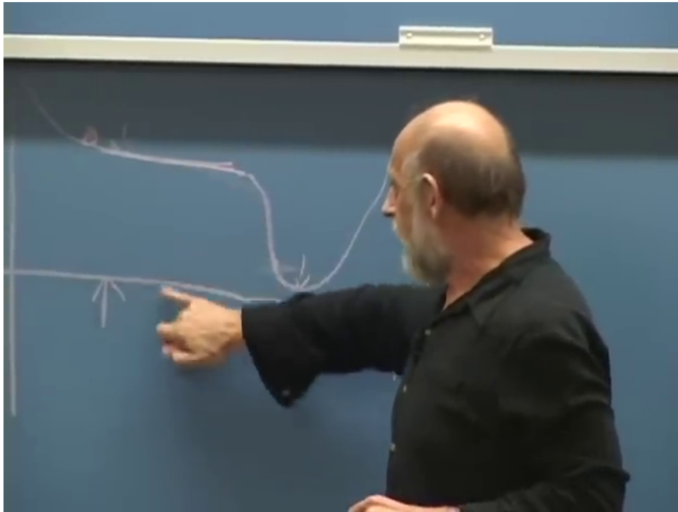
Figure 1.1: Qualitative inflaton potential with a broad plateau, a steep drop, and a low minimum.
