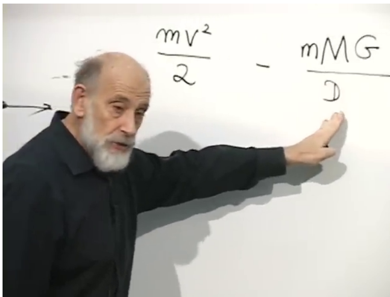
Figure 2.5: At small outward speed, the negative potential term dominates the total energy.
