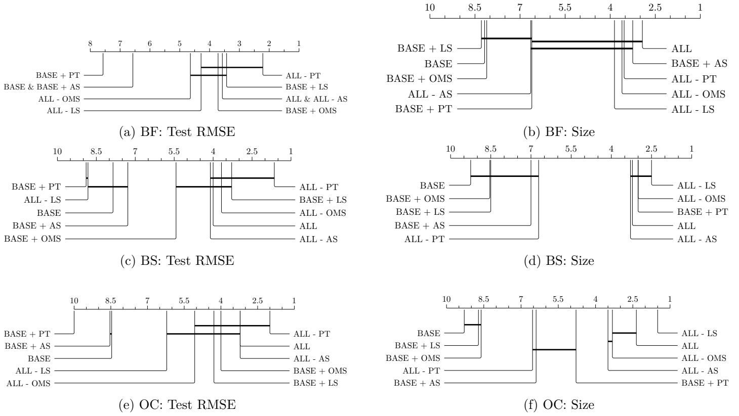
Figure 1: Critical difference diagrams for the Best Fitness (BF), Optimal Compromise (OC) and Best Size (BS) models; where A.: ALL and B.: BASE. (SLIM+ABS)
