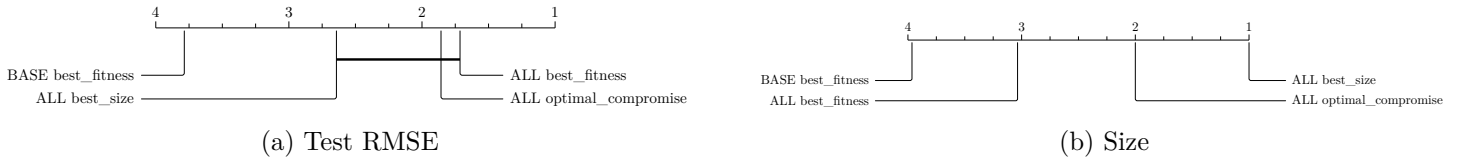
Figure 2: Critical Difference Diagram comparing the final models (BF, BS and OC) found by the ALL variant with the SLIM (BASE) BF model. (SLIM+ABS)
