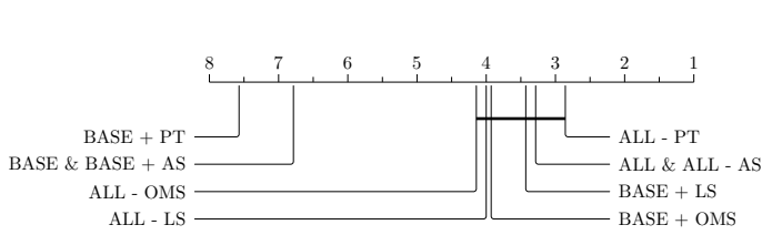
(a) BF: Test RMSE
