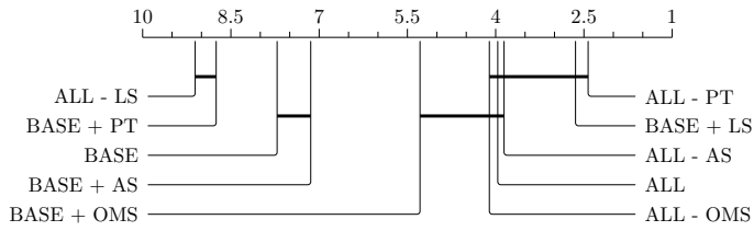
(c) BS: Test RMSE
