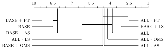
(e) OC: Test RMSE
