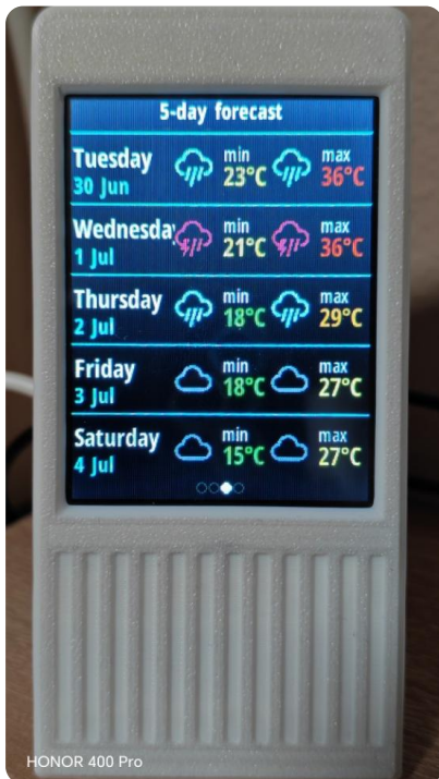
5-day forecast
