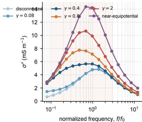
a Finite contacts reshape the SIP spectrum
