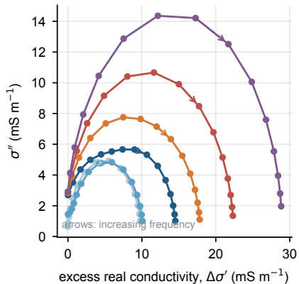
b Distinct complex-plane trajectories
