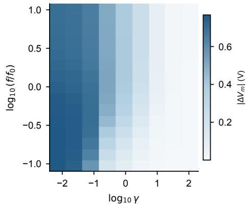
c Contact voltage collapses toward equipotentiality
