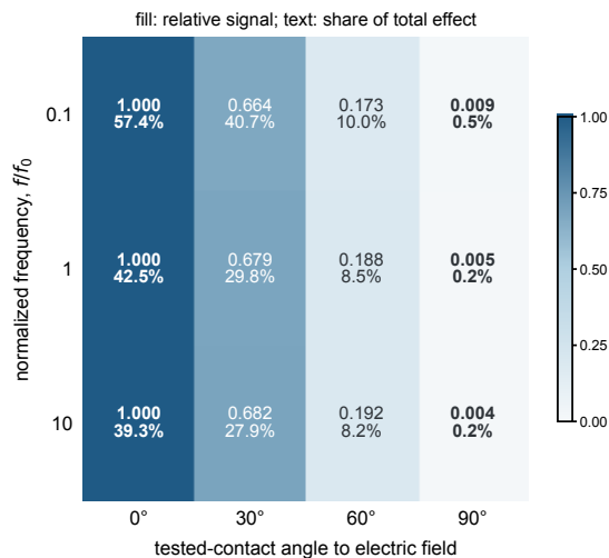
a Selected FEM response: signal falls with angle
