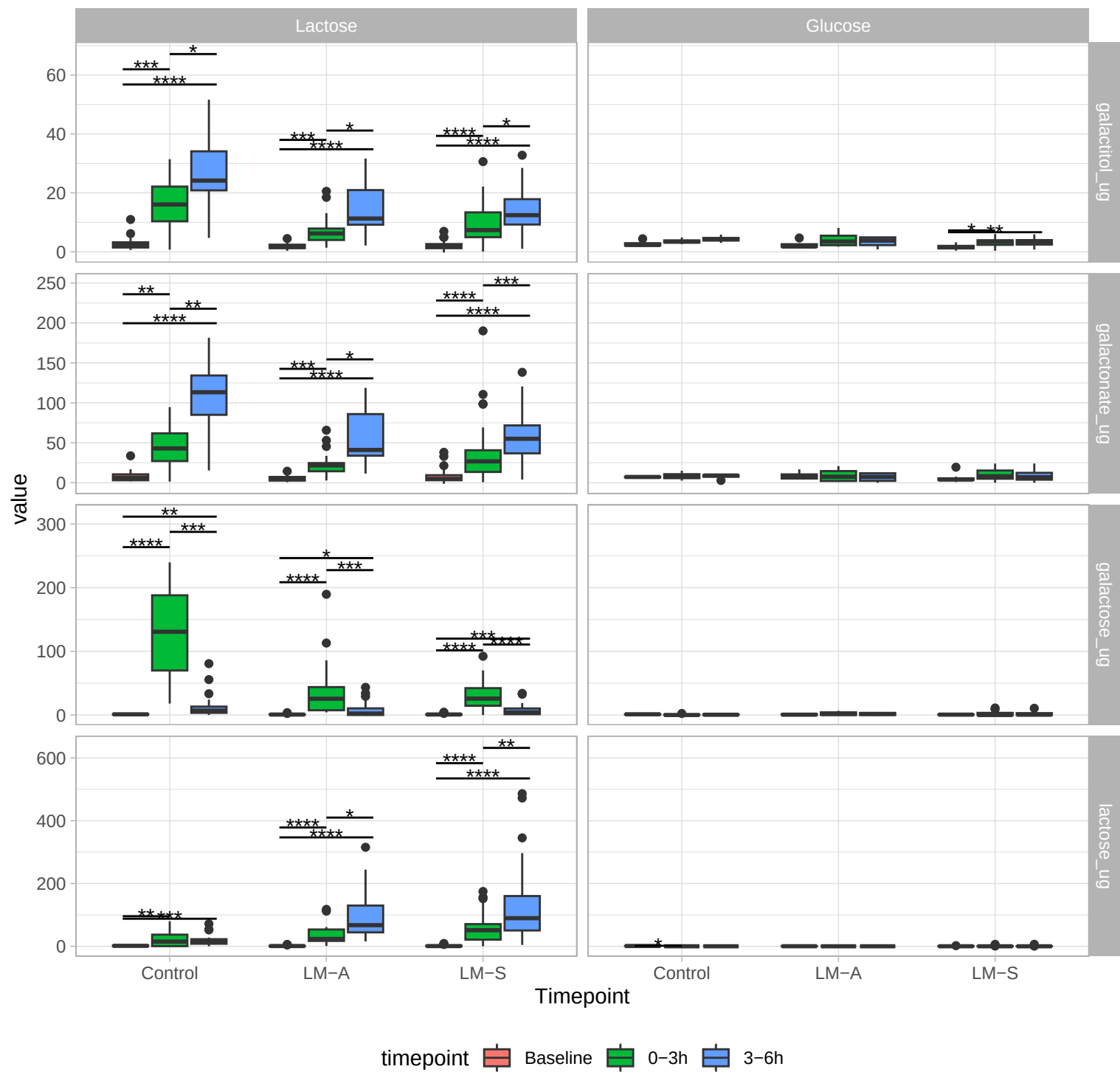
Distribution of metabolite values per study group, timepoint, and treatment
