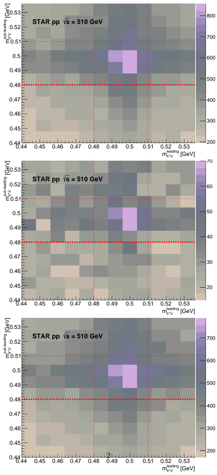
Figure 1: Leading vs sub-leading mass distribution
