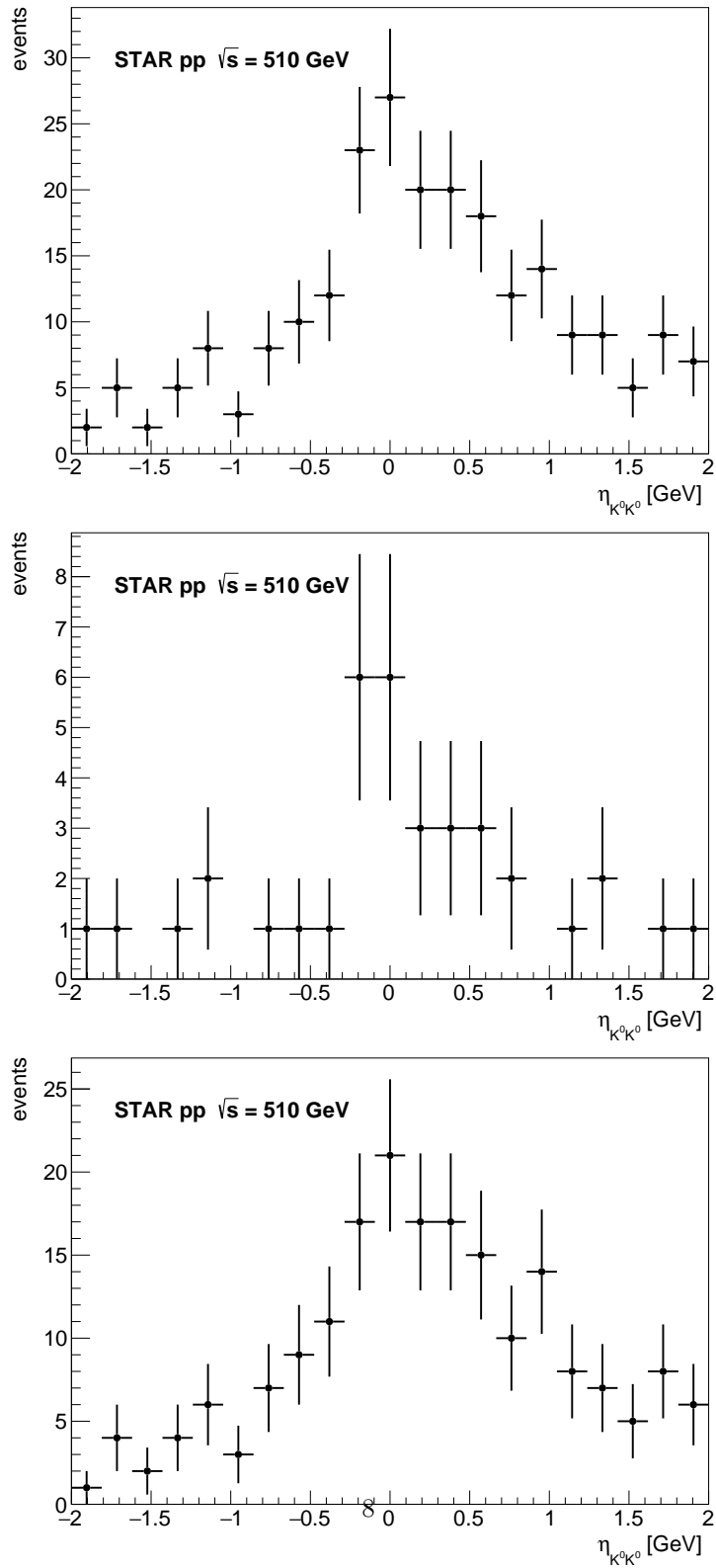
Figure 6: K^0\bar{K}^0 \eta
