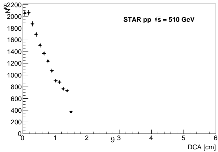
Figure 7: DCA
