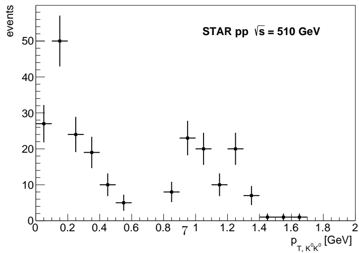
Figure 5: K^0 K^0 p_T
