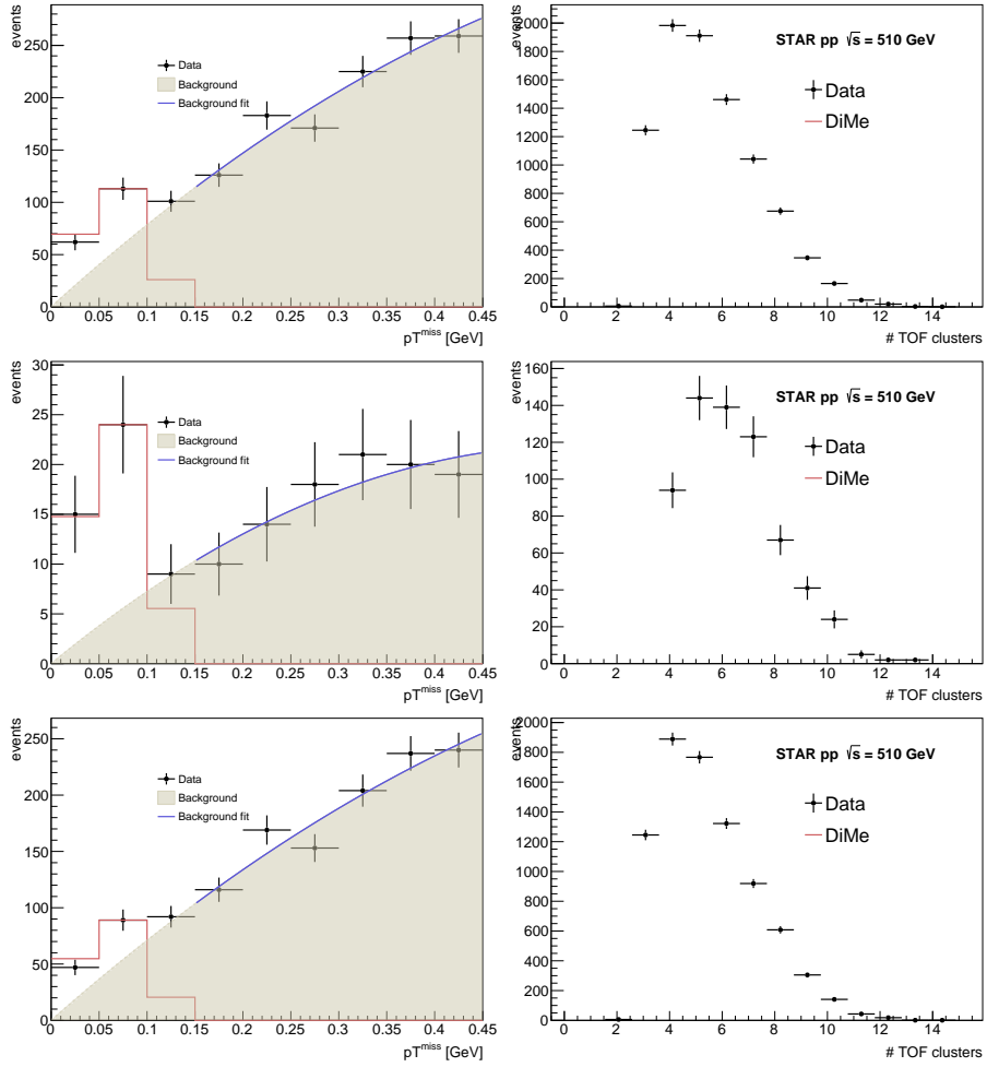
Figure 2: p_T^{miss} GeV and N_{cluster}
