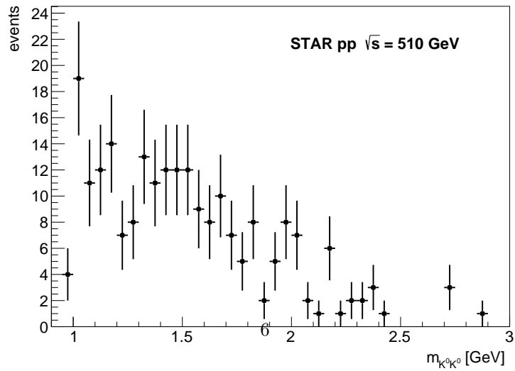
Figure 4: K0K0 mass
