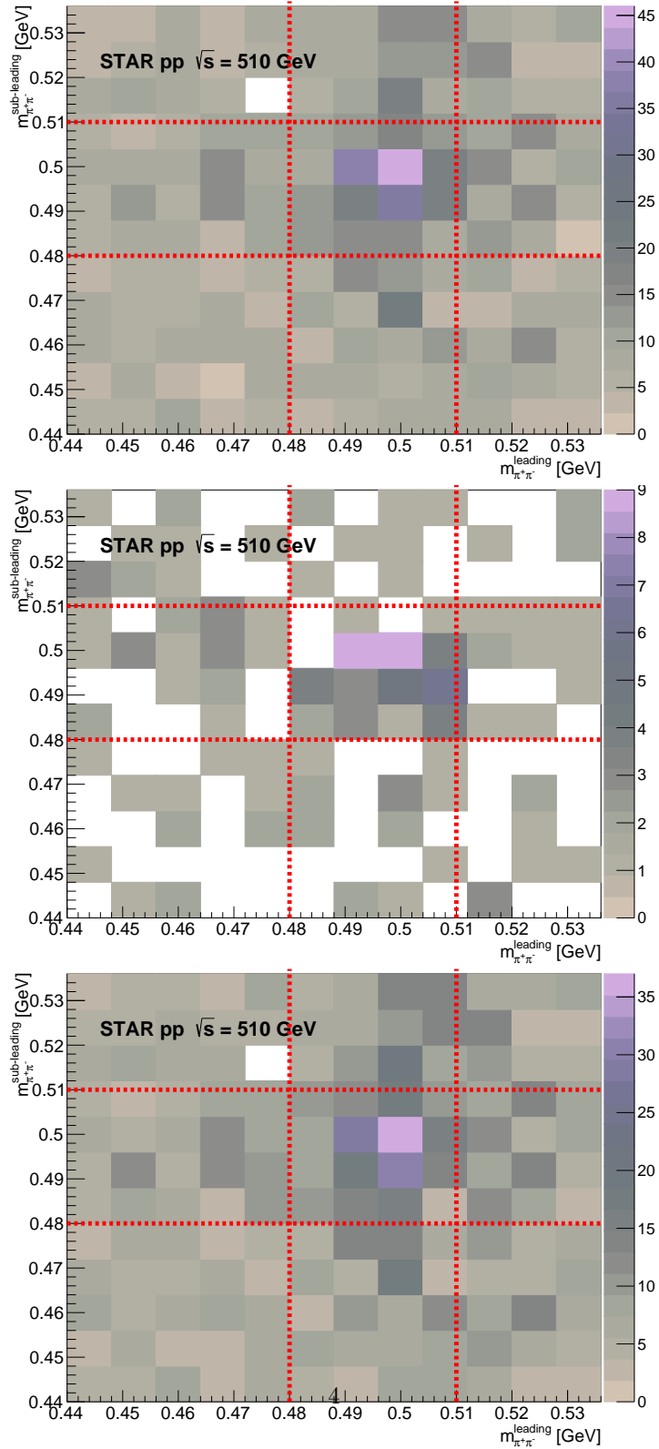
Figure 3: Leading vs sub-leading mass distribution with p_T^{\text{miss}} < 0.15 GeV and N_{\text{cluster}} \leq 9
