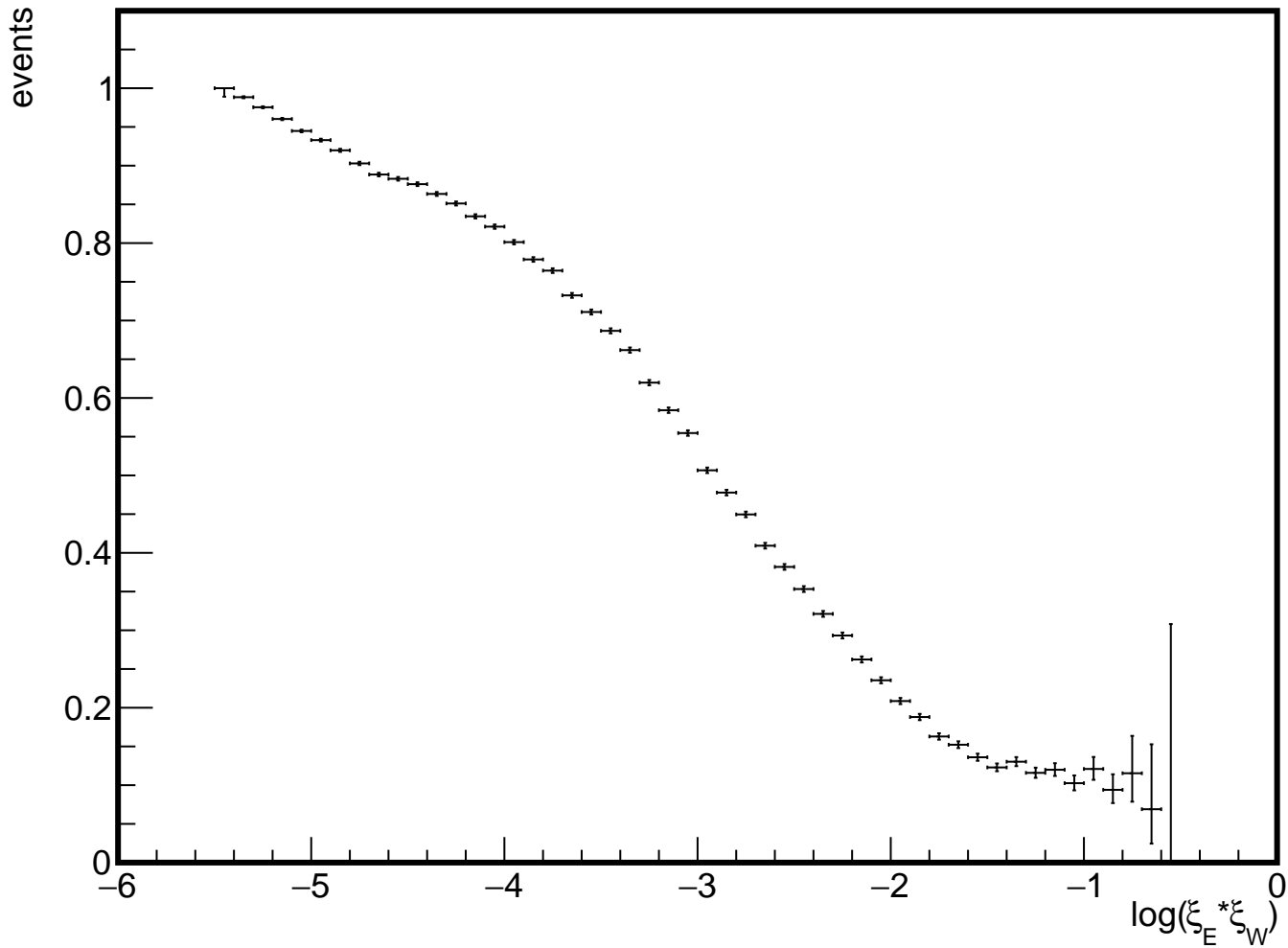
Effect of BBCL cut on \log(\xi_E * \xi_W) with |\ln(\xi_E / \xi_W)| < 4 condition
