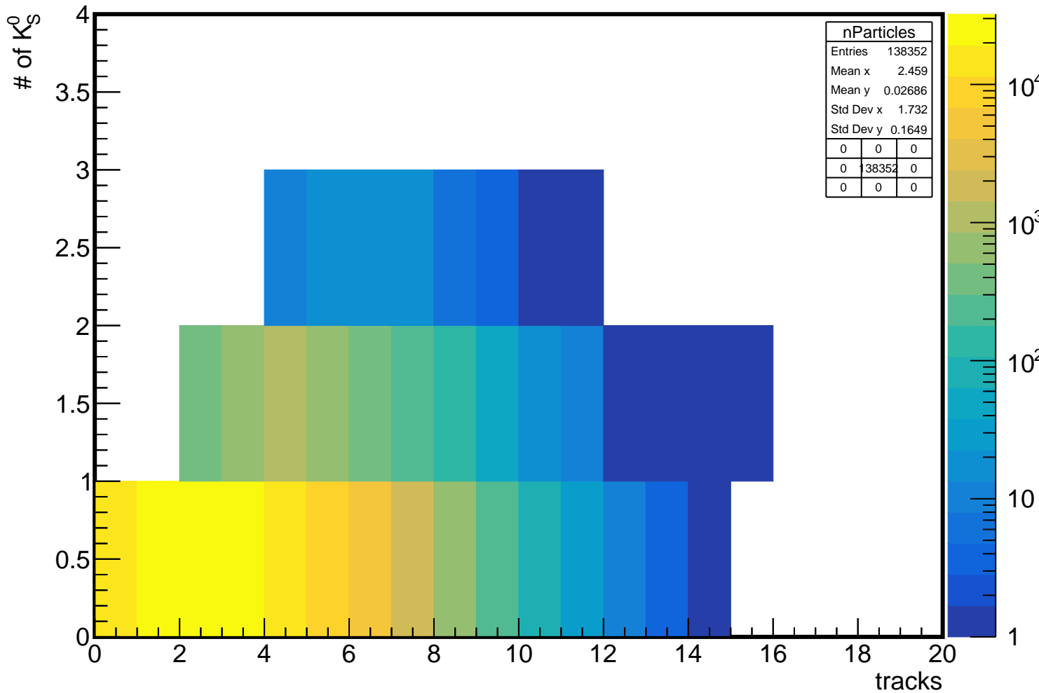
Number of tracks visible in TPC vs number of detected K_S^0 with both \xi conditions
