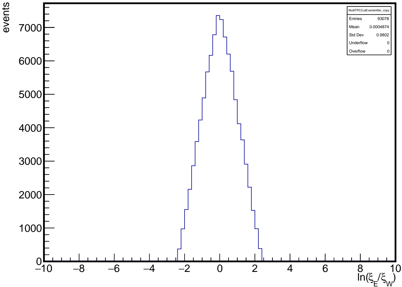
Effect of TPC cut on \ln(\xi_E/\xi_W) with 0.007 < \xi_{E,W} < 0.08 conditions
