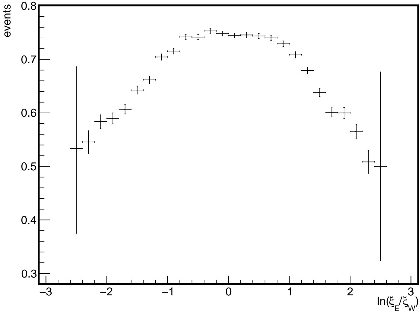
Effect of BBCL cut on \ln(\xi_E/\xi_W) with 0.007 < \xi_{E,W} < 0.08 conditions
