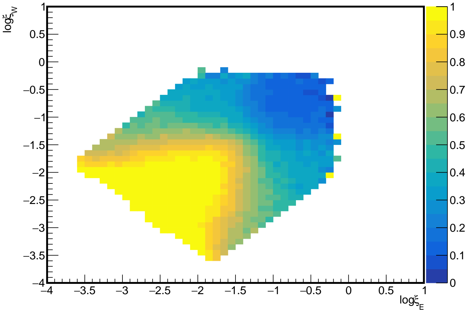
Effect of BBCL cut on \log \xi_E vs \log \xi_W with |\ln(\xi_E/\xi_W)| < 4 condition
