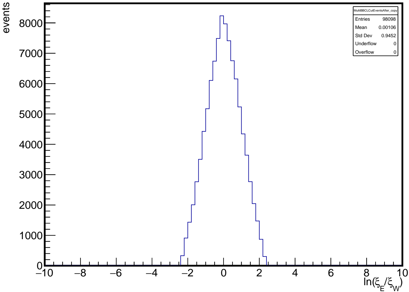
Effect of BBCL cut on \ln(\xi_E/\xi_W) with 0.007 < \xi_{E,W} < 0.08 conditions
