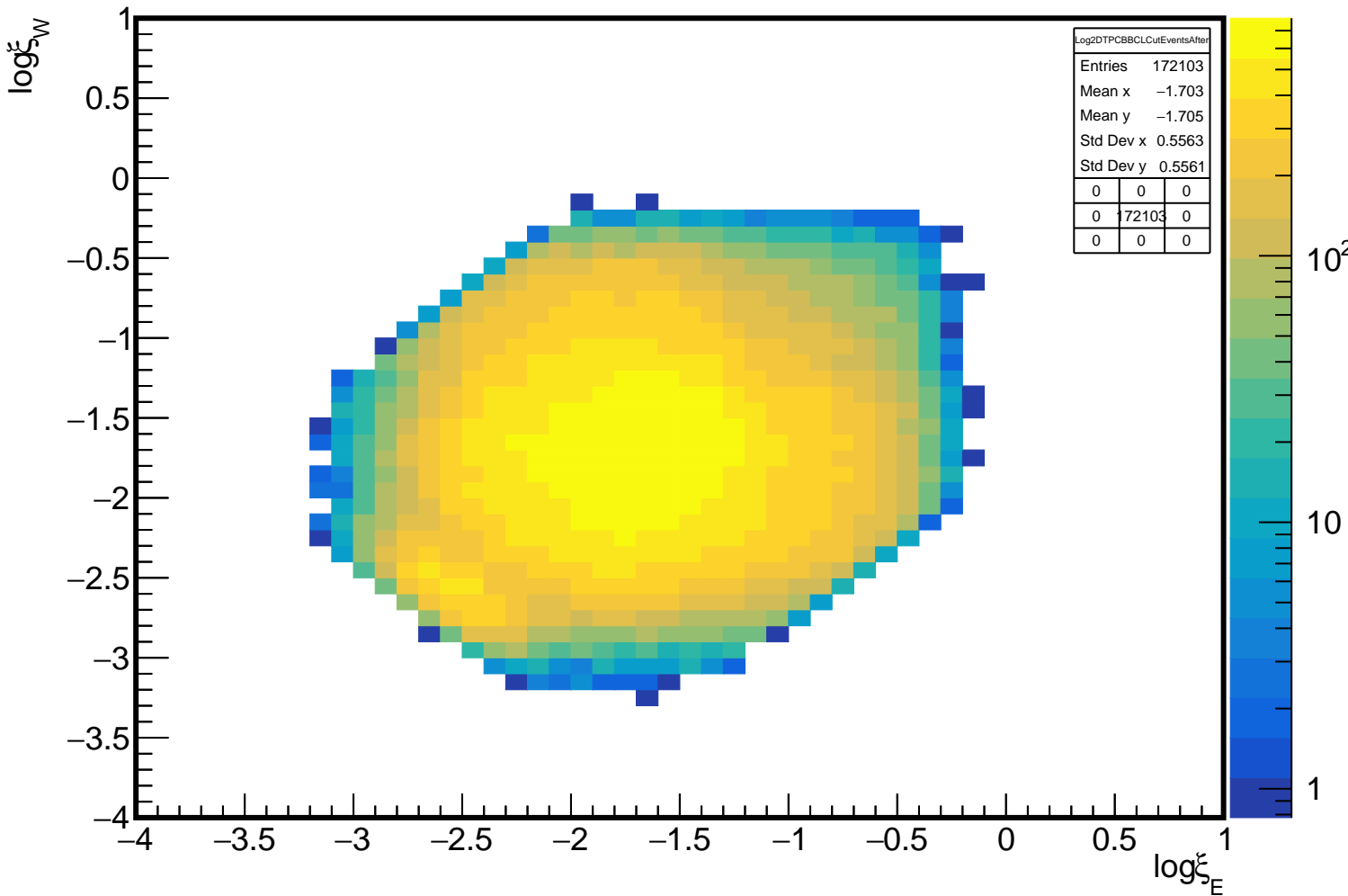
Effect of TPC and BBCL cut on \log \xi_E vs \log \xi_W with |\ln(\xi_E/\xi_W)| < 4 condition
