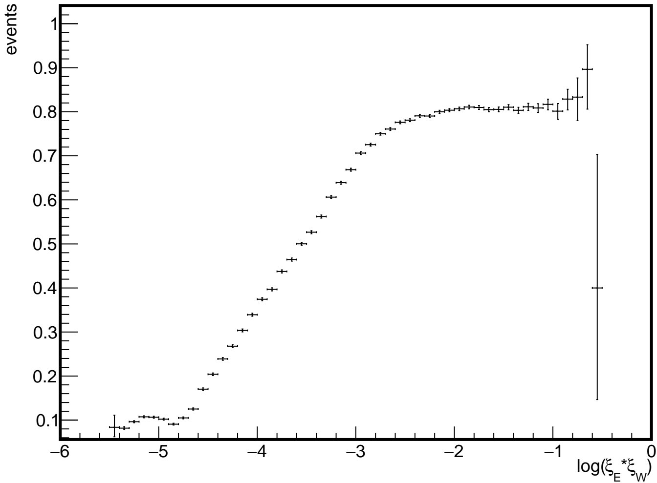
Effect of TPC cut on \log(\xi_E^* \xi_W) with |\ln(\xi_E/\xi_W)| < 4 condition
