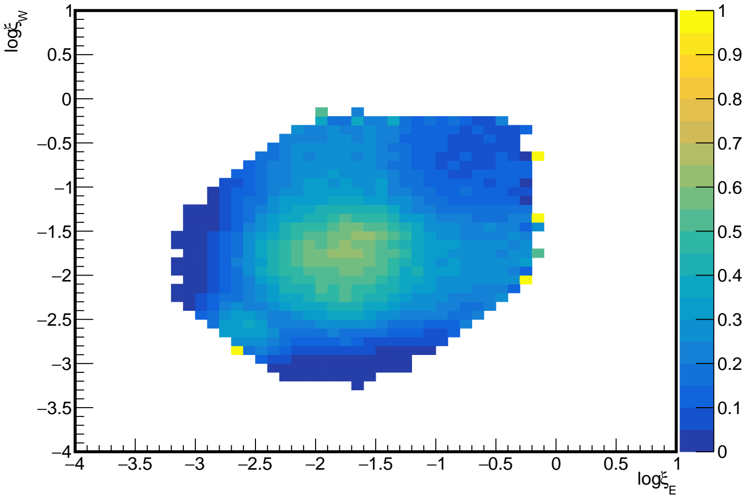
Effect of TPC and BBCL cuts on \log \xi_E vs \log \xi_W with |\ln(\xi_E/\xi_W)| < 4 condition
