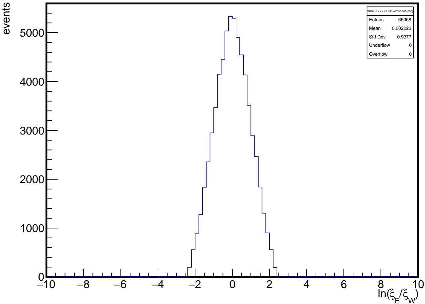
Effect of TPC and BBCL cuts on \ln(\xi_E/\xi_W) with 0.007 < \xi_{E,W} < 0.08 conditions
