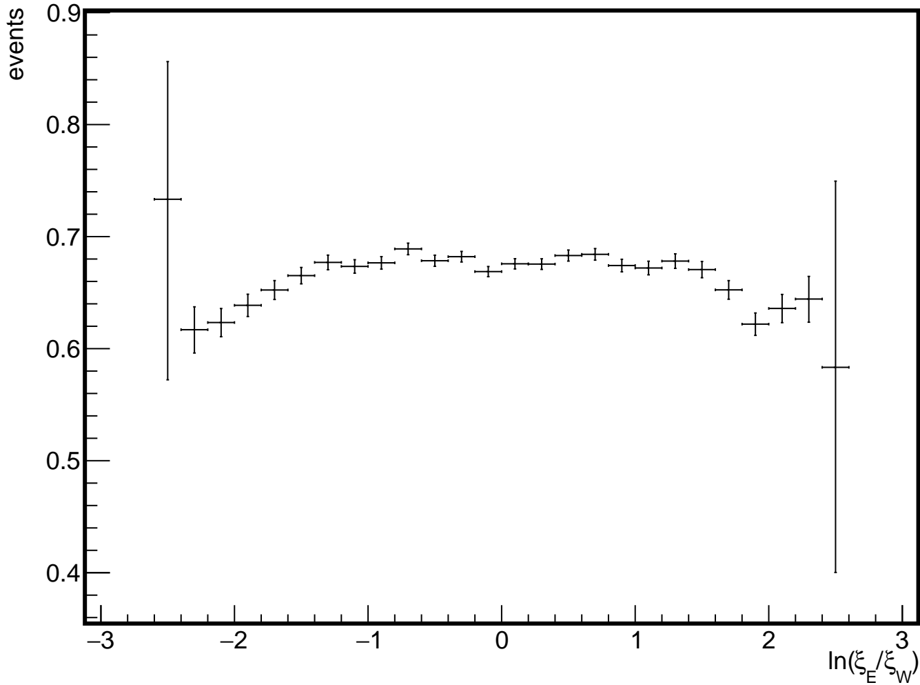
Effect of TPC cut on \ln(\xi_E/\xi_W) with 0.007 < \xi_{E,W} < 0.08 conditions
