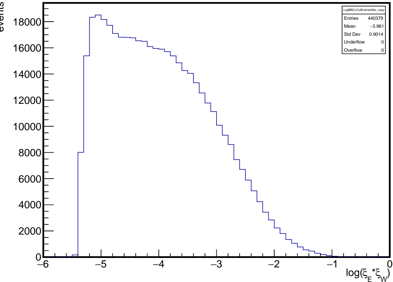
Effect of BBCL cut on \log(\xi_E * \xi_W) with |\ln(\xi_E / \xi_W)| < 4 condition
