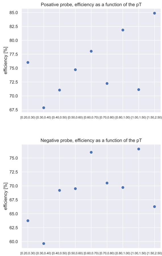
Figure 1: Efficiency as a function of p_T for positive (top) and negative (bottom) probe.
