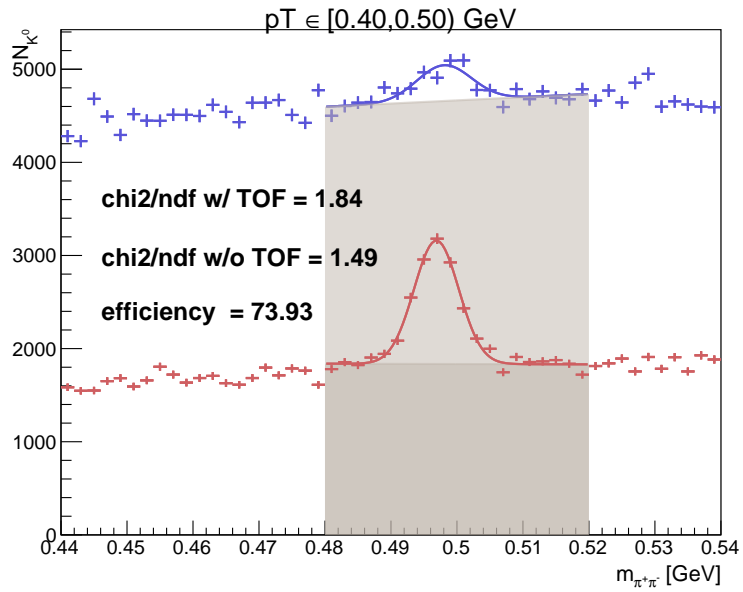
Figure 2: linear fit 0.48-0.52 GeV
