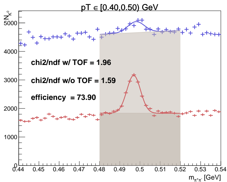
Figure 4: quadratic fit 0.48-0.52 GeV
