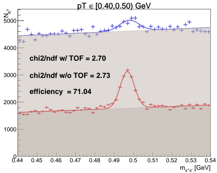
Figure 1: linear fit 0.44-0.53 GeV
