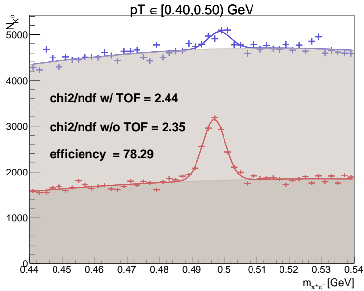
Figure 3: quadratic fit 0.44-0.54 GeV
