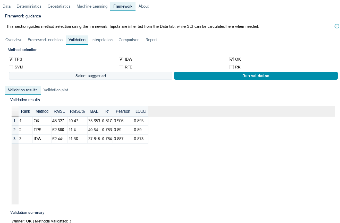
Figure 20: Framework validation tab showing method selection, the validation results table, and the validation summary for the selected methods.
