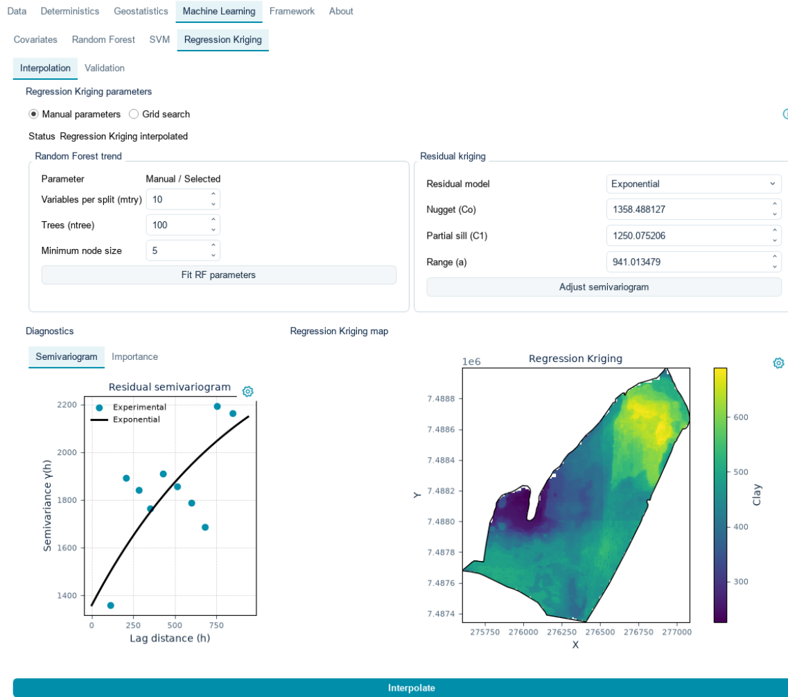
Figure 15: Regression Kriging tab showing the Random Forest trend settings, residual kriging parameters, residual semivariogram, and final RK interpolation map.
