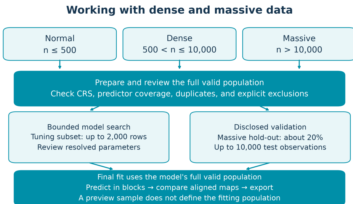
Figure 30: Processing flow for dense and massive data: distinguish tuning, validation, final fitting, and display samples.
