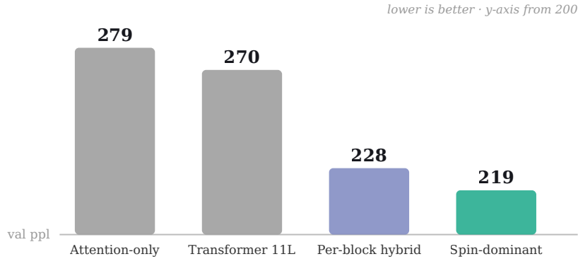
Figure 6. Param-matched ablation ( \sim 37 – 46 M, same corpus and budget, single seed). Spin as the token-mixer (219) beats the attention-only baseline (279) by \sim 21\% , and the larger per-block hybrid (228) and param-matched transformer (270), with fewer or equal weights.
