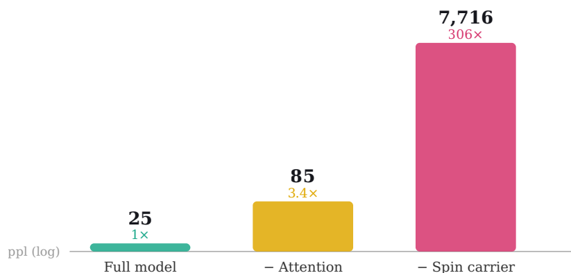
Figure 8. Causal ablation on the 284M spin-dominant model (log scale). Zeroing the spin carrier sends validation perplexity from 25 to 7,716 (306×); zeroing attention only to 85 (3.4×). The carrier is the load-bearing core.
