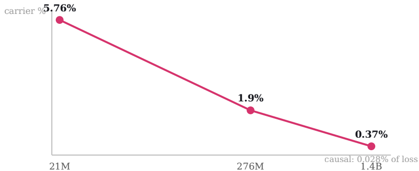
Figure 5. A fixed single spin carrier is one d-shaped layer, so as depth and width grow its parameter share collapses (5.76%→1.90%→0.37% from 21M to 1.4B) and its measured causal contribution falls to 0.028% of the loss at 1.4B the motivation for making the carrier the core rather than a side-channel.
