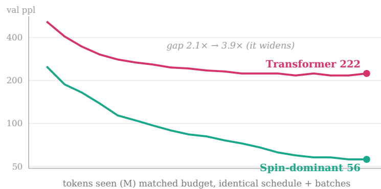
Figure 7. Learning curves at matched \sim 37\text{M} , identical schedule and batches, each at its range-test learning rate (spin 6.7\text{e-}3 , transformer 1.0\text{e-}4 ), to 117M tokens. Both converge, but to very different floors: the transformer plateaus at \sim 222 while the spin-dominant model descends to \sim 56 , so the gap widens through training and settles at 3.9\times ( 2.1\times \rightarrow 3.9\times ). This directly answers the natural objection that the short-budget gap is just "the transformer hasn't trained yet": given a full schedule at its own best learning rate, the transformer descends and then flattens it does not close the gap. (Small-scale, single-seed.)
