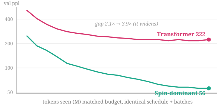
Figure 4. Learning curves at matched \sim 37\text{M} , identical schedule and batches, each at its range-test learning rate (spin 6.7\text{e-}3 , transformer 1.0\text{e-}4 ), to 117\text{M} tokens. Both converge, but to very different floors: the transformer plateaus at \sim 222 while the spin-dominant model descends to \sim 56 , so the gap widens through training and settles at 3.9\times ( 2.1\times \rightarrow 3.9\times ). This directly answers the natural objection that the short-budget gap is just "the transformer hasn't trained yet": given a full schedule at its own best learning rate, the transformer descends and then flattens it does not close the gap. (Small-scale, single-seed.)
