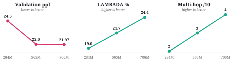
Figure 9. Progression across the three grown sizes. Validation perplexity falls, and LAMBADA (the most fluency-dependent benchmark) and the greedy multi-hop battery both rise monotonically the design improves consistently as it grows and trains, with the largest gains on the tokens-limited axes.
