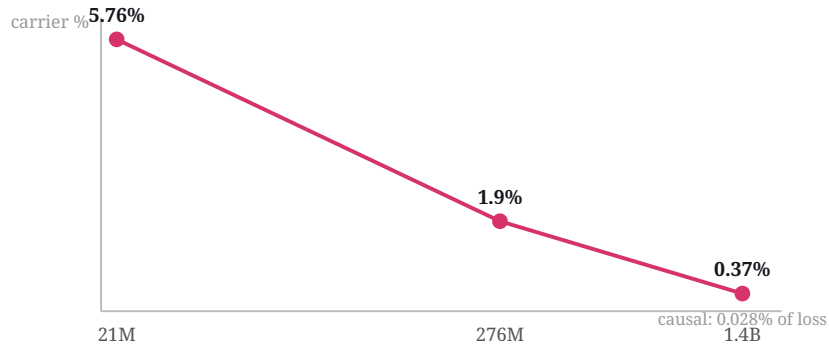
Figure 5. A fixed single spin carrier is one d-shaped layer, so as depth and width grow its parameter share collapses ( 5.76\% \rightarrow 1.90\% \rightarrow 0.37\% from 21M to 1.4B) and its measured causal contribution falls to 0.028% of the loss at 1.4B the motivation for making the carrier the core rather than a side-channel.
