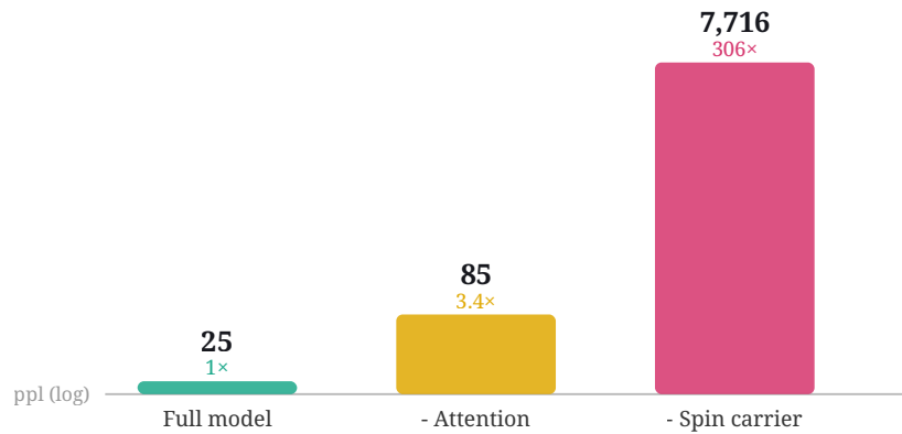
Figure 4. Causal ablation on the 284M spin-dominant model (log scale). Zeroing the spin carrier sends validation perplexity from 25 to 7,716 (306×); zeroing attention only to 85 (3.4×). The carrier is the load-bearing core.
